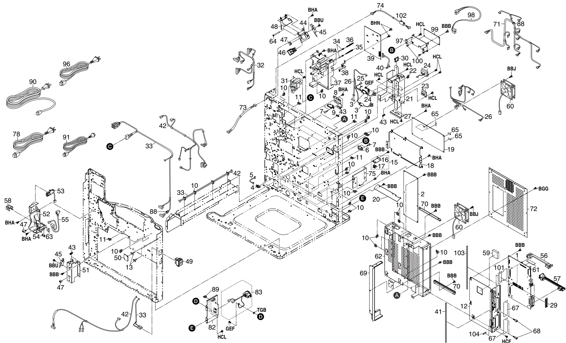
FIG. 17 Electrical components
