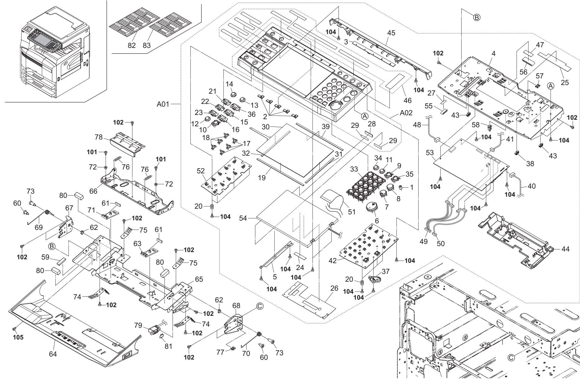
FIG. 23 Operation Section
