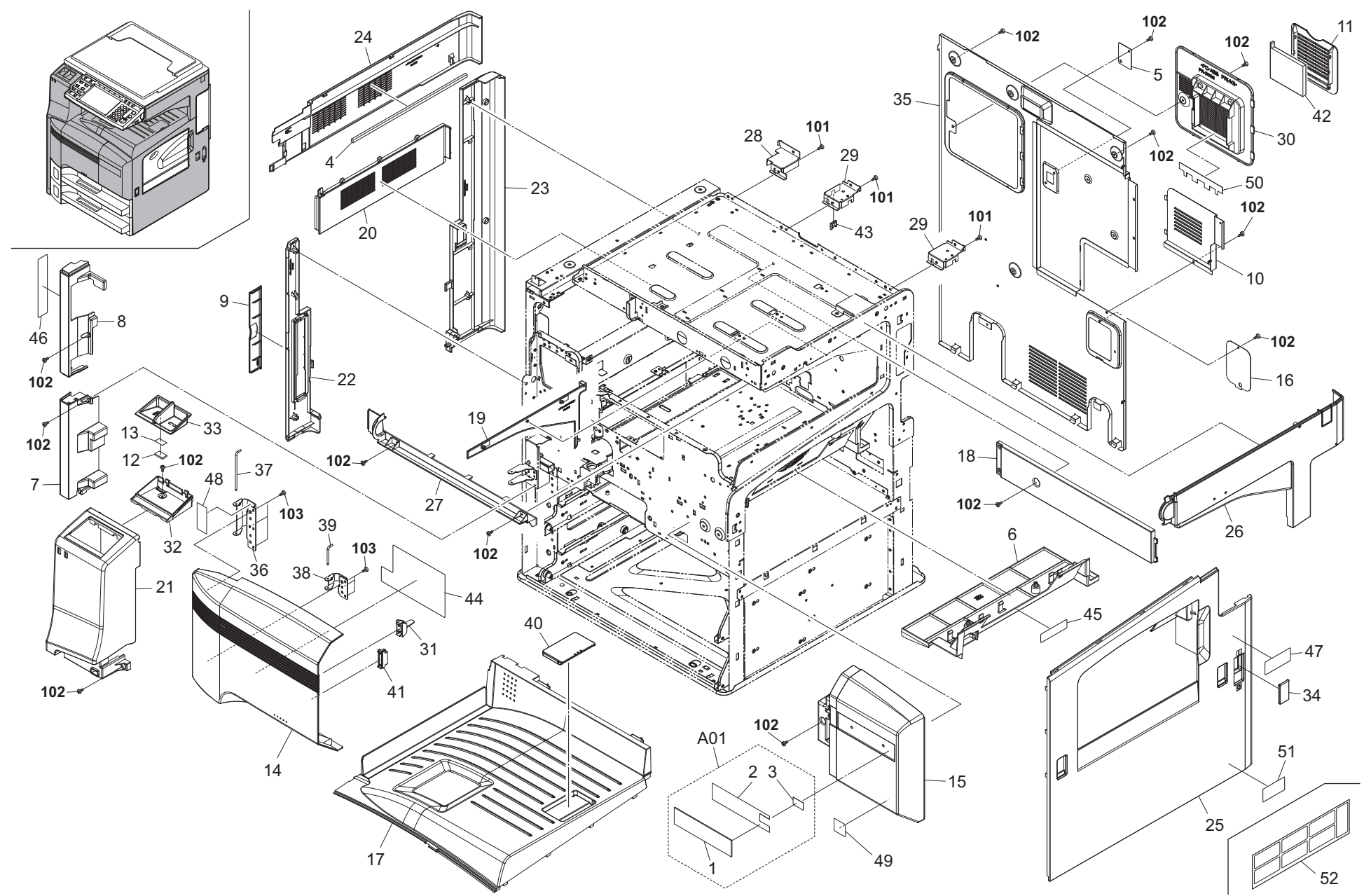
FIG. 1 Covers
