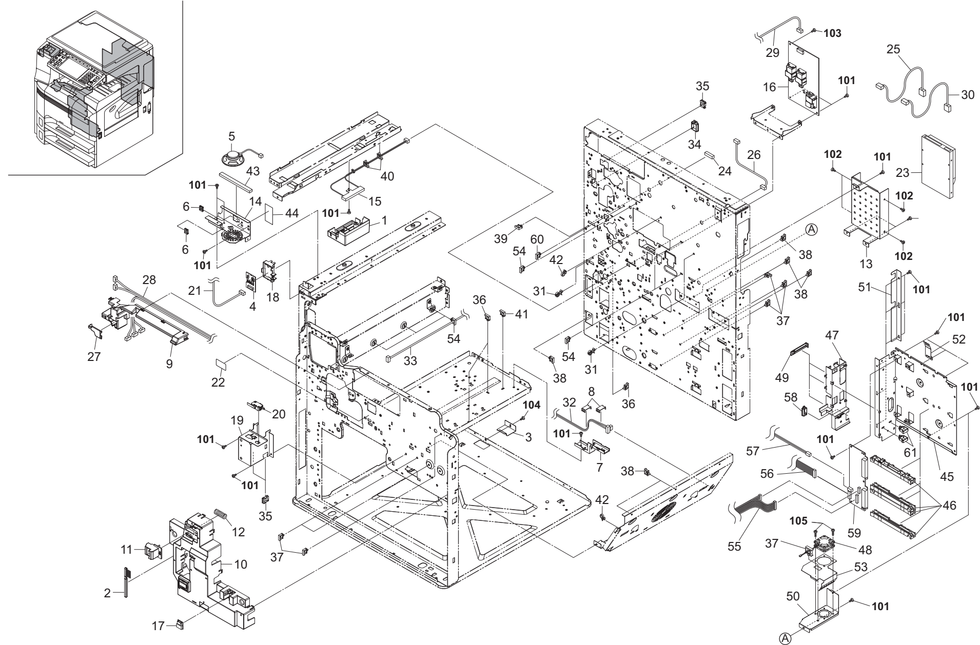
FIG. 22 Electrical Components 2
