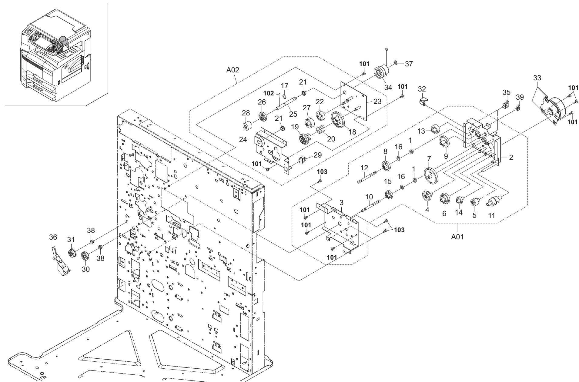
FIG. 16 Drive Section 2
