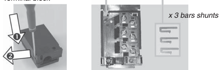
Terminal block
