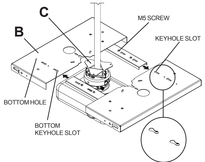
DETAIL 1
