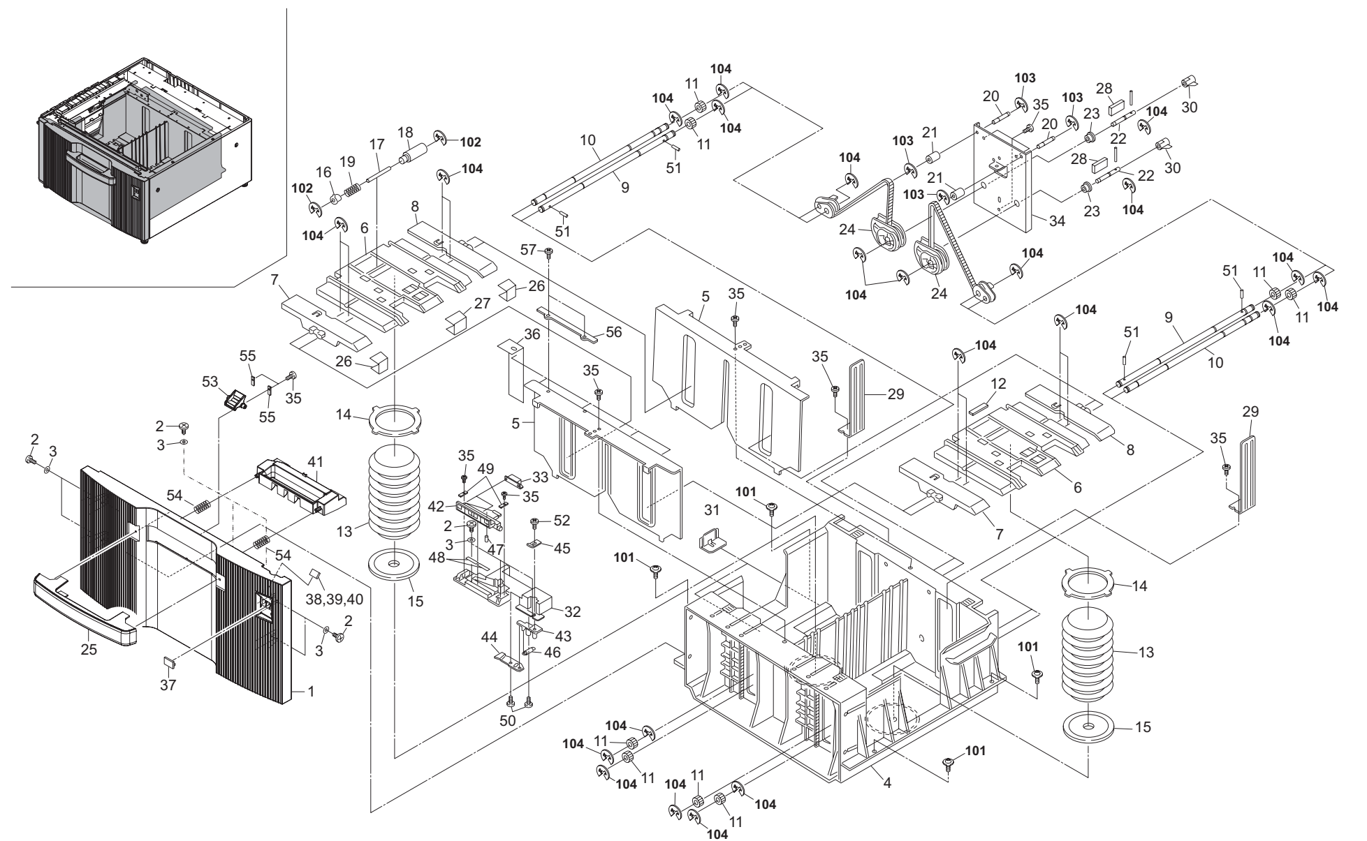
FIG. 2 Paper Cassette
