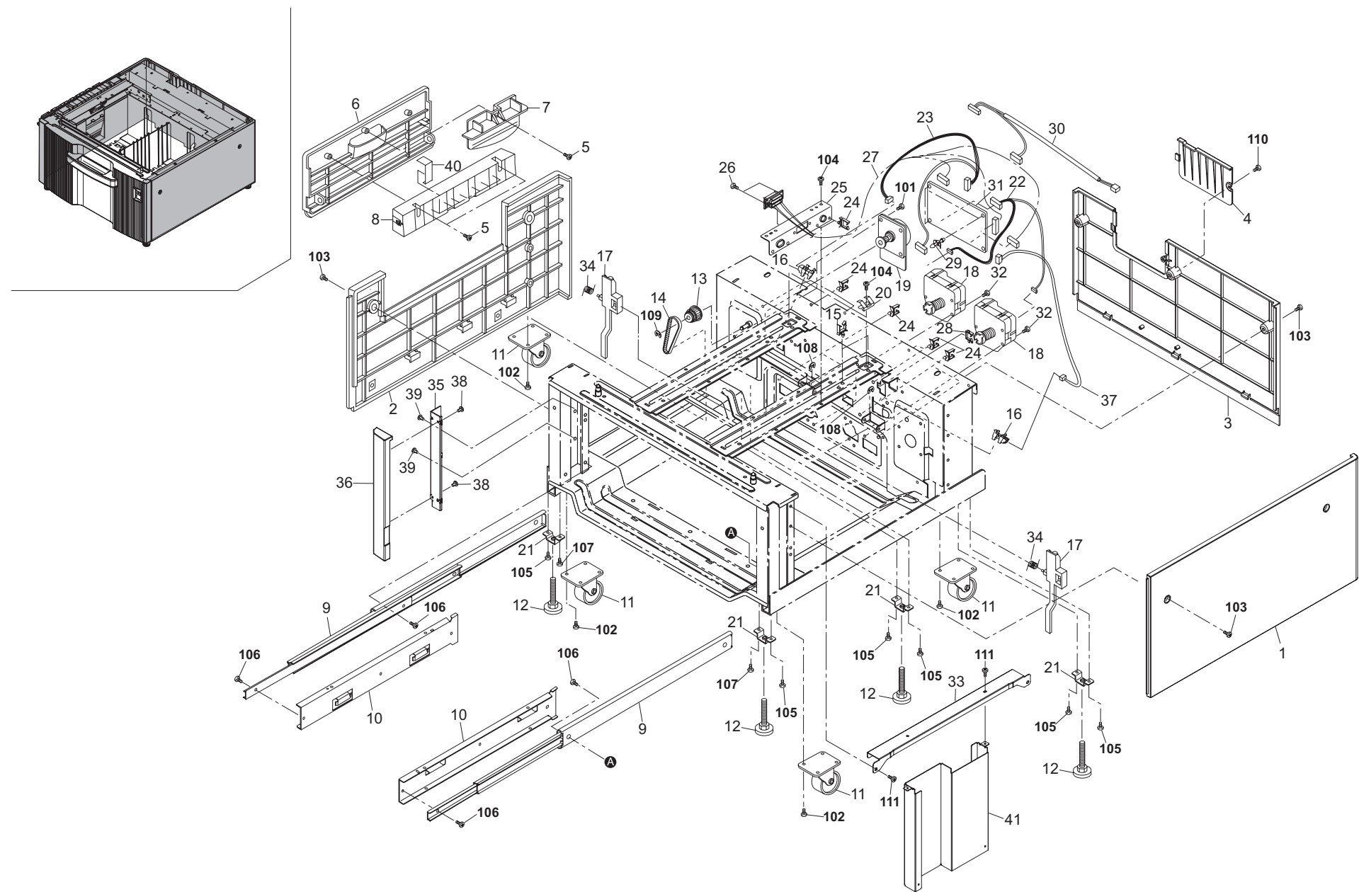
FIG. 1 Covers
