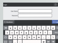
Login screen
