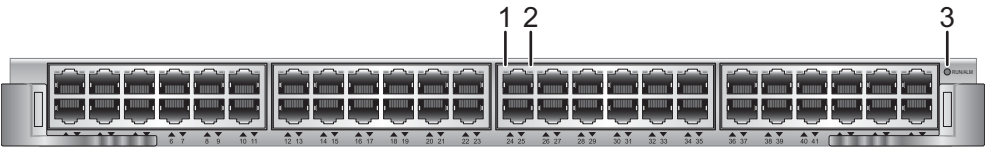
Figure 6-70 Indicators on the ES1D2G48TBC0 panel
