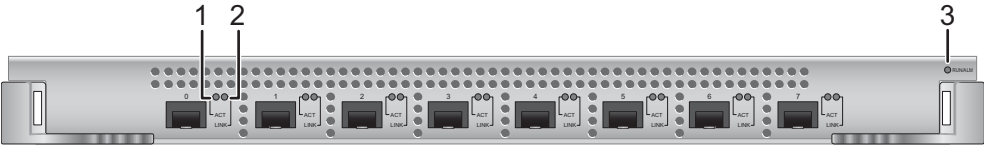
Figure 6-109 Indicators on the ES1D2X08SED4/ES1D2X08SED5 panel
