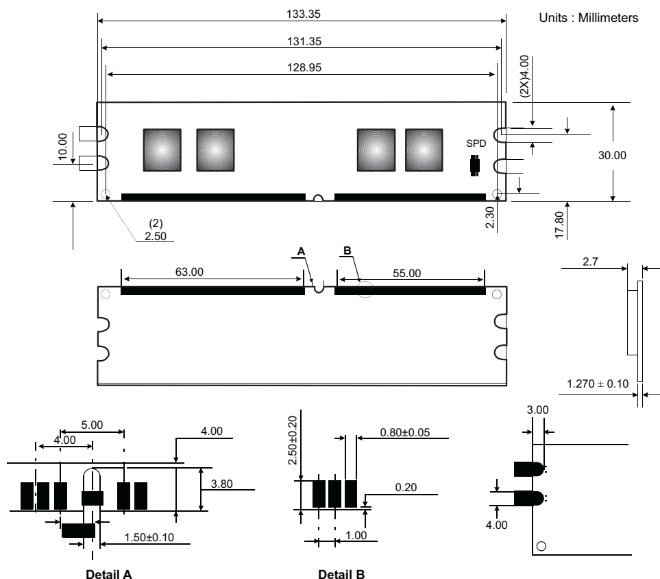
Figure 1: KVR533D2N4/256 240-Pin DIMM
