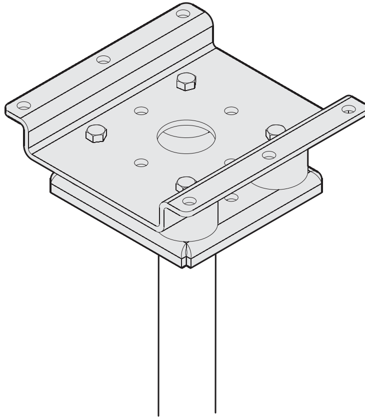
Ceiling Plate with Flex Joints
