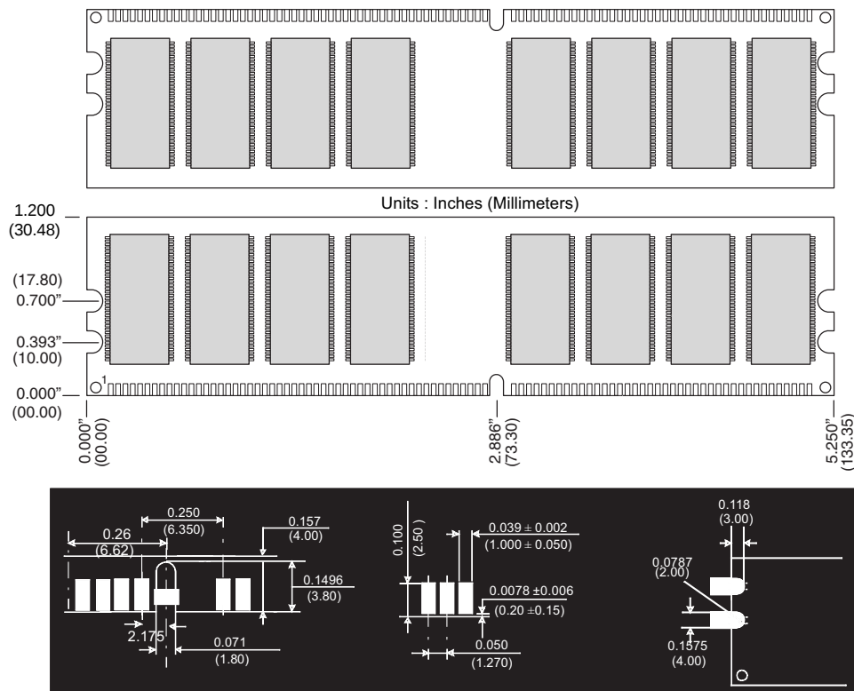
Figure 1: KVR266/512R 184-Pin DDR SDRAM Module
