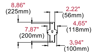
CEILING PLATE
