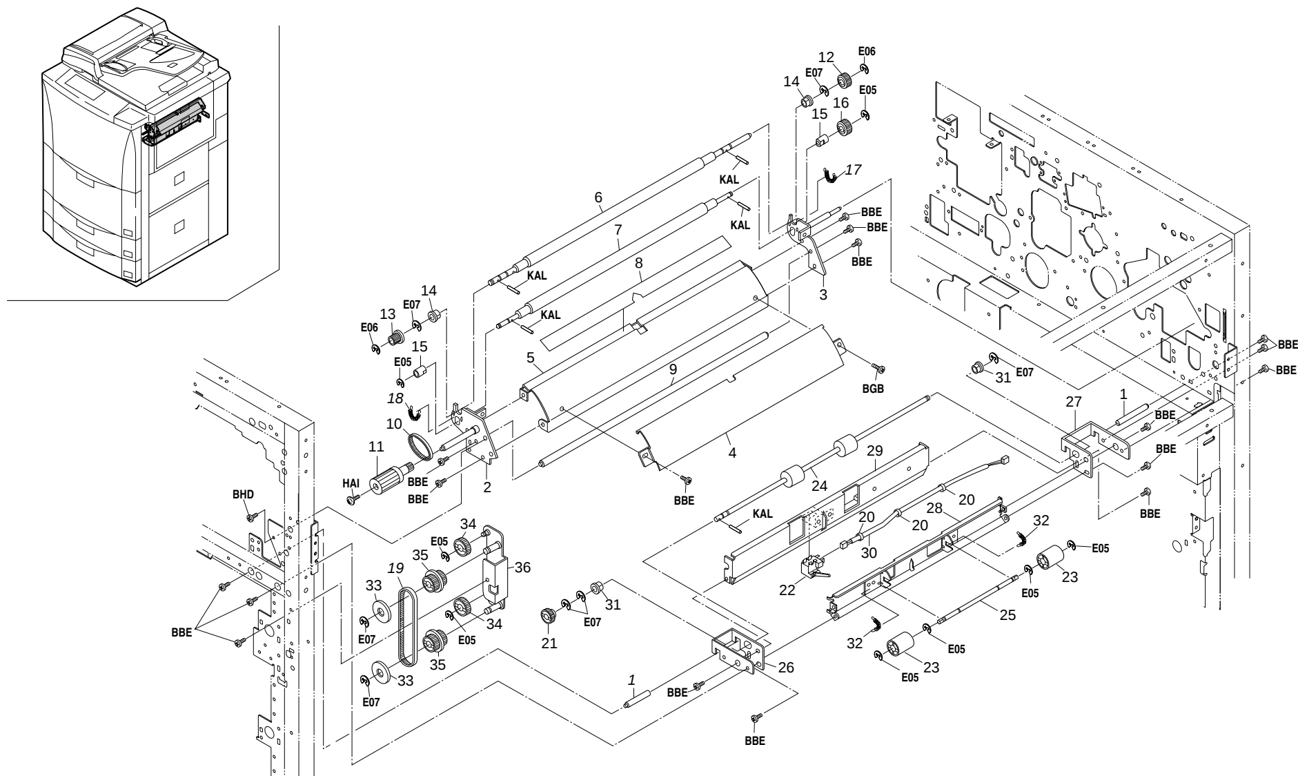
FIG.10 PAPER FEED-IN SECTION IV
