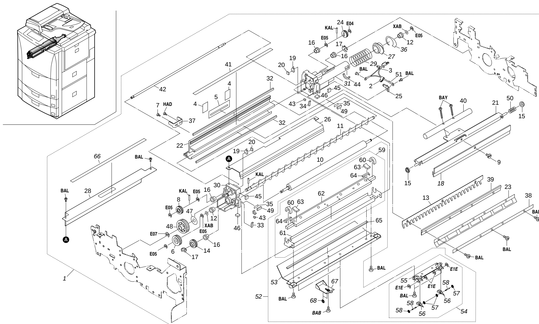
FIG.21 CLEANING SECTION I
