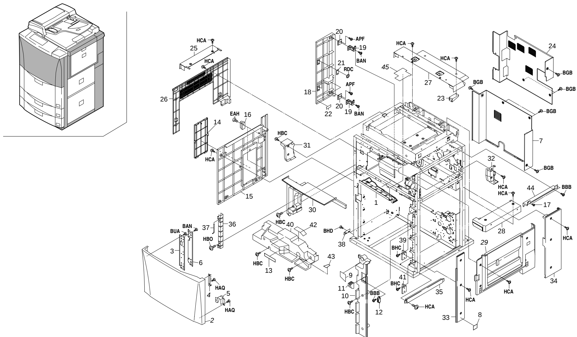
FIG. 1 EXTERIOR COVERS
