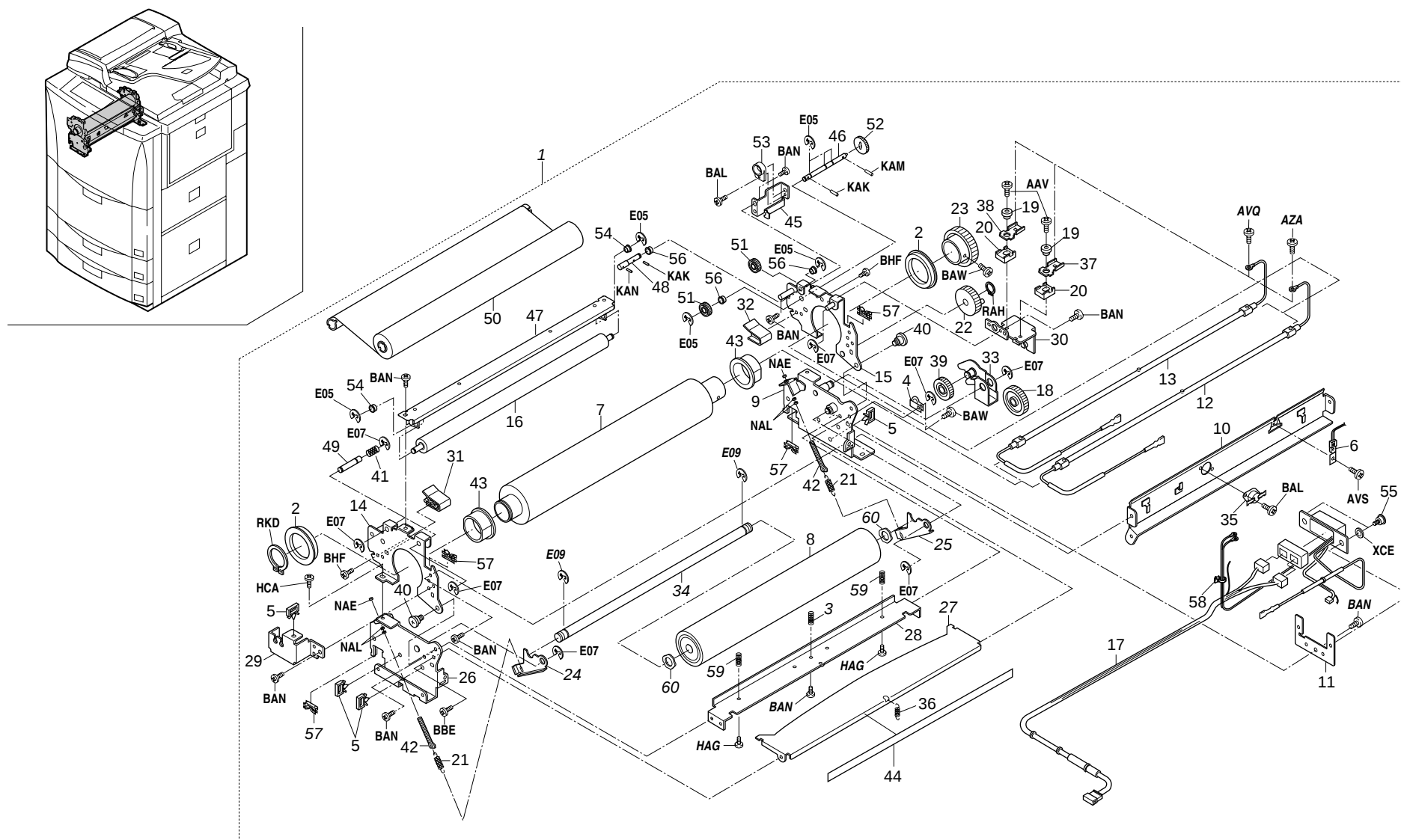
FIG.25 FIXING SECTION II
