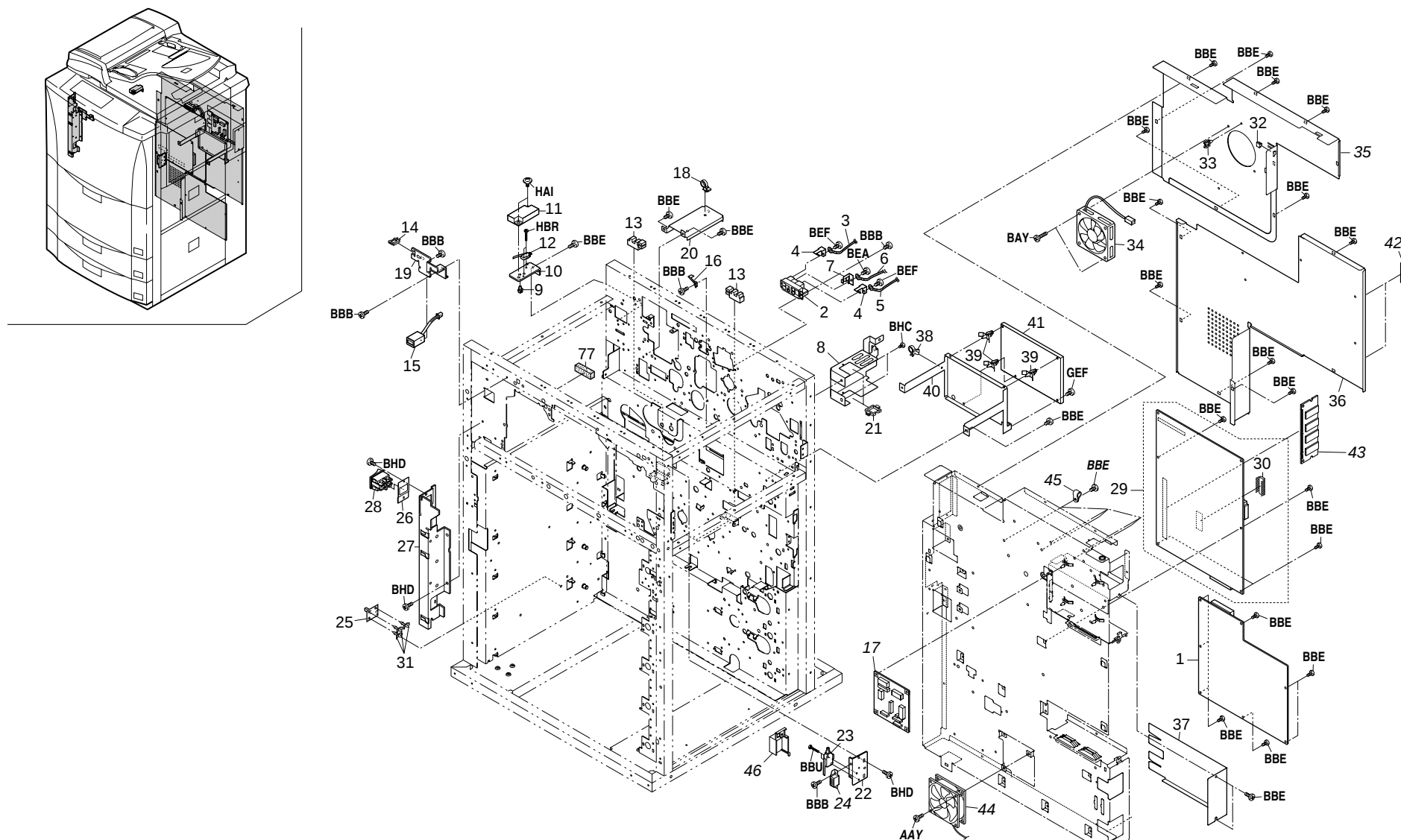
FIG.35 ELECTRICAL COMPONENTS II
