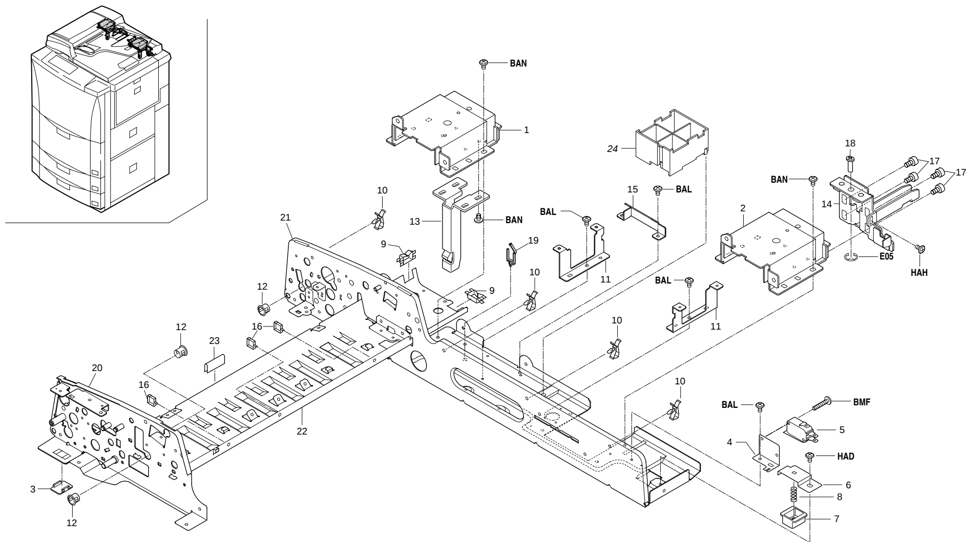
FIG.42 FRAMES (DP)
