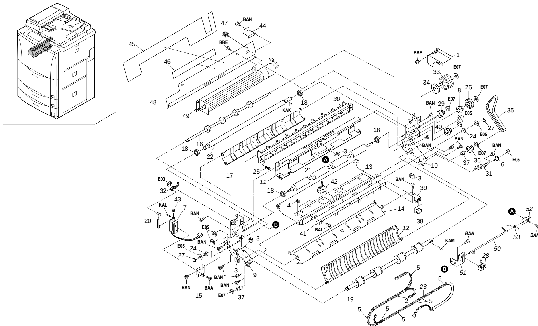
FIG.32 REVERSING SECTION
