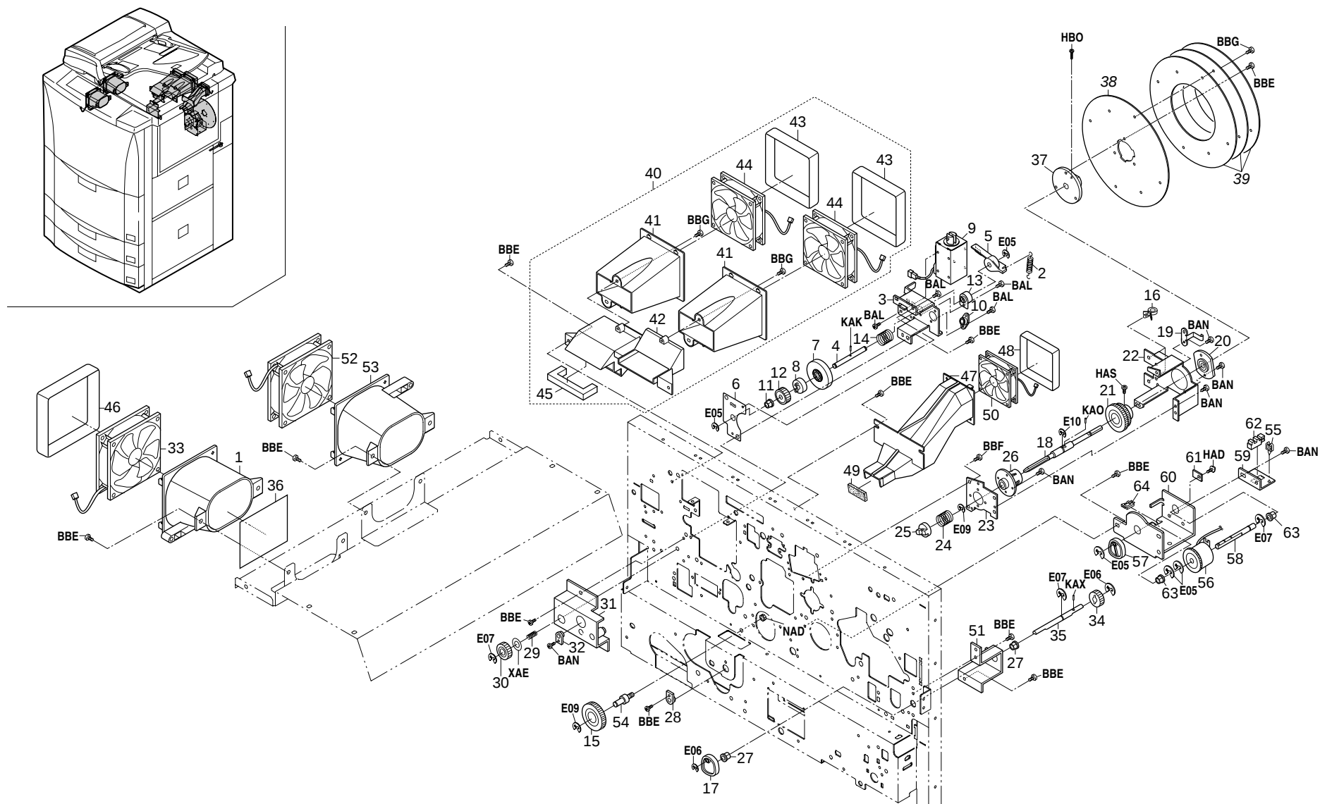
FIG.27 DRIVING, COOLING SECTION II
