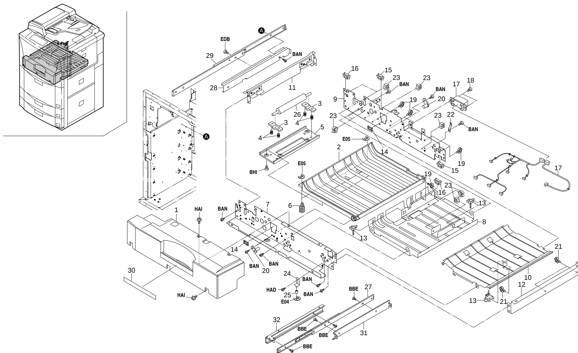
FIG.29 DUPLEX UNIT I
