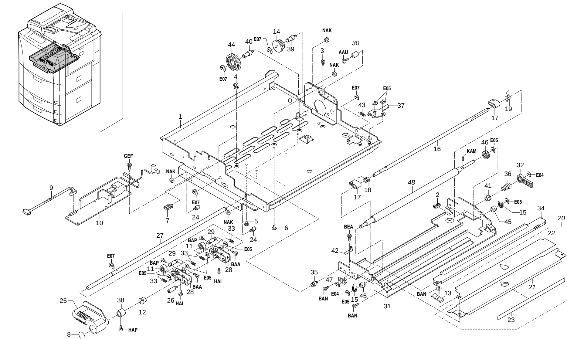
FIG.13 PAPER CONVEYING SECTION II
