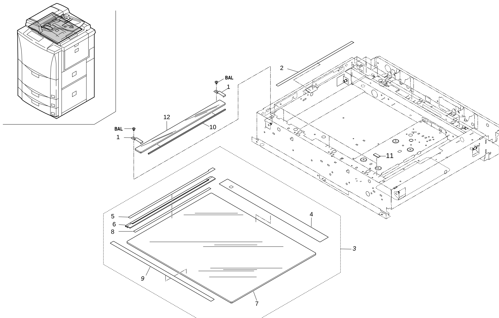
FIG.15 OPTICAL SECTION II
