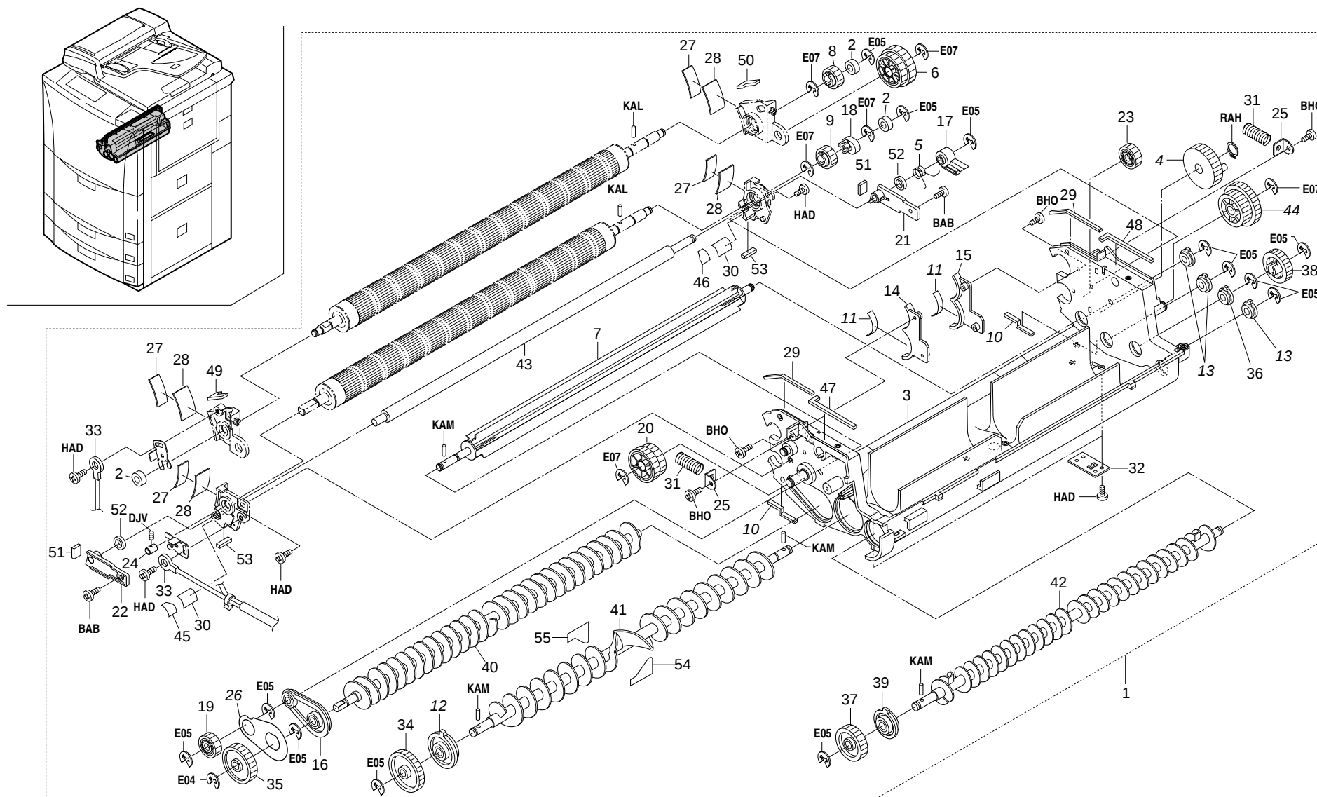
FIG.19 DEVELOPING SECTION II
