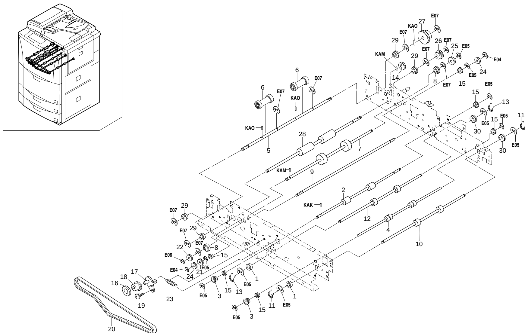
FIG.31 DUPLEX UNIT III
