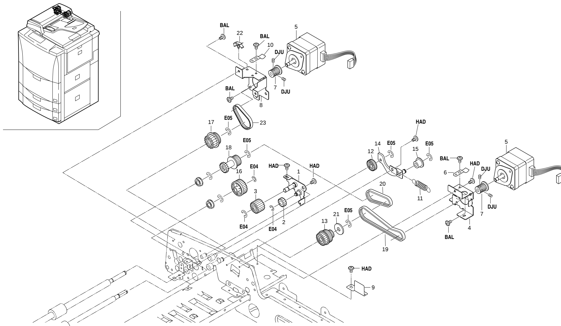
FIG.47 DRIVING SECTION (DP)
