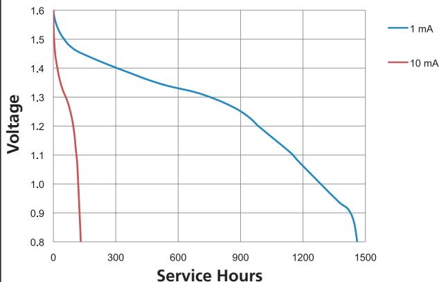
Plus Power AAA Constant Current
