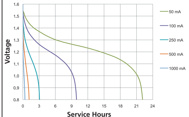
Plus Power AAA Constant Current
