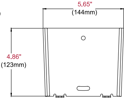
WALL PLATE DETAIL
