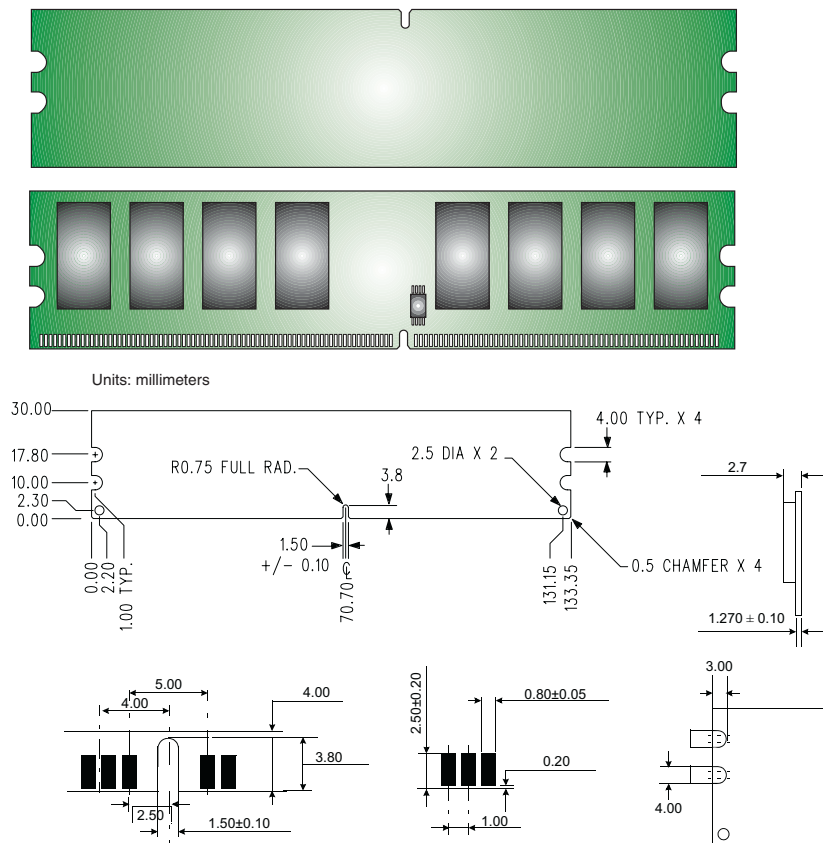
Figure 1: KVR800D2N6K2/1G 240-Pin DIMM Kit
