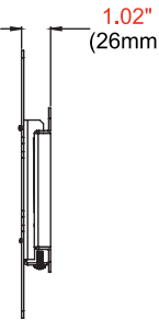
SIDE VIEW VESA 100/200
