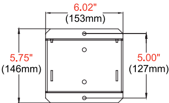
WALL PLATE DETAIL
