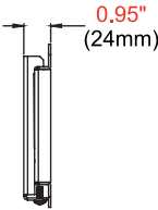
SIDE VIEW VESA 75/100
