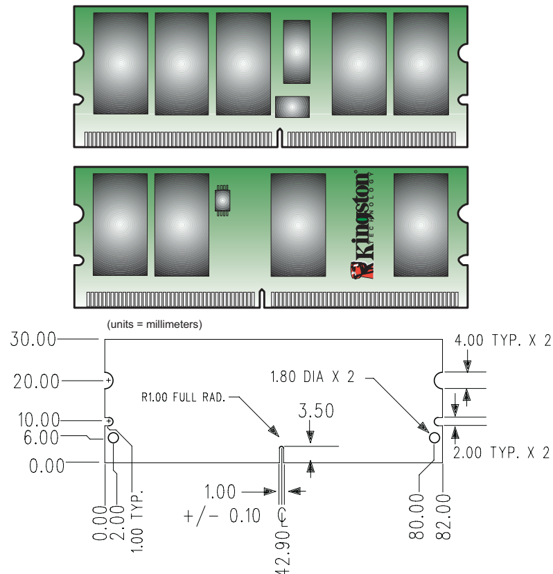
Figure 1: KVR400D2M3/256 244-Pin MiniDIMM
