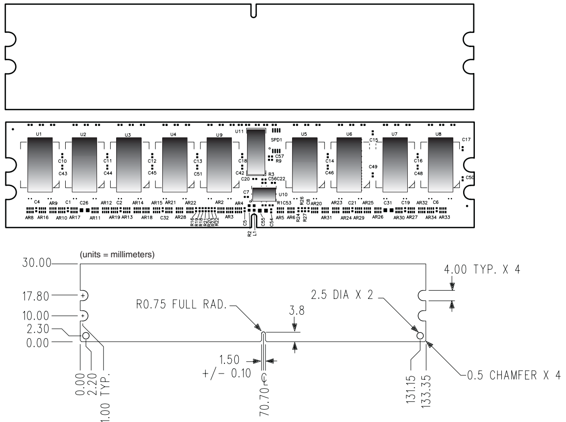
Figure 1: KVR533D2S8R4K2/2G 240-Pin DIMM
