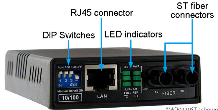
*MCM110ST2 shown
