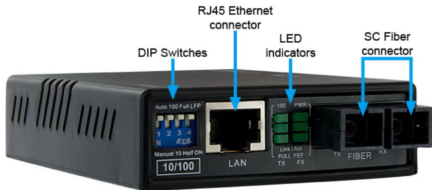
*MCM110SC2 shown
