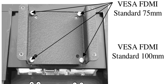
Figure 2. 75mm Bracket Installation
