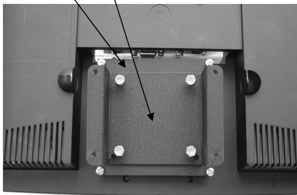
Figure 4. 100mm to 75mm Installation
