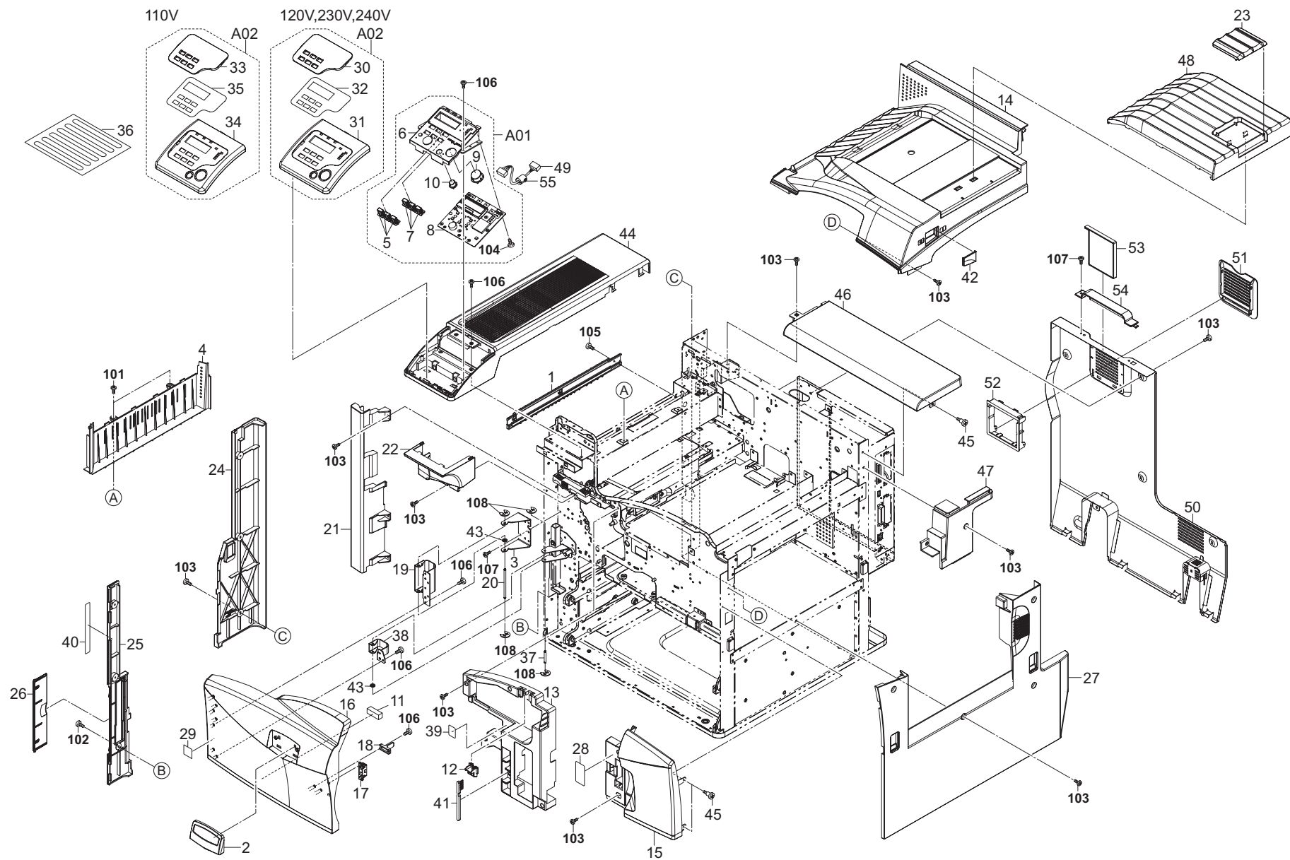
FIG. 1 Covers
