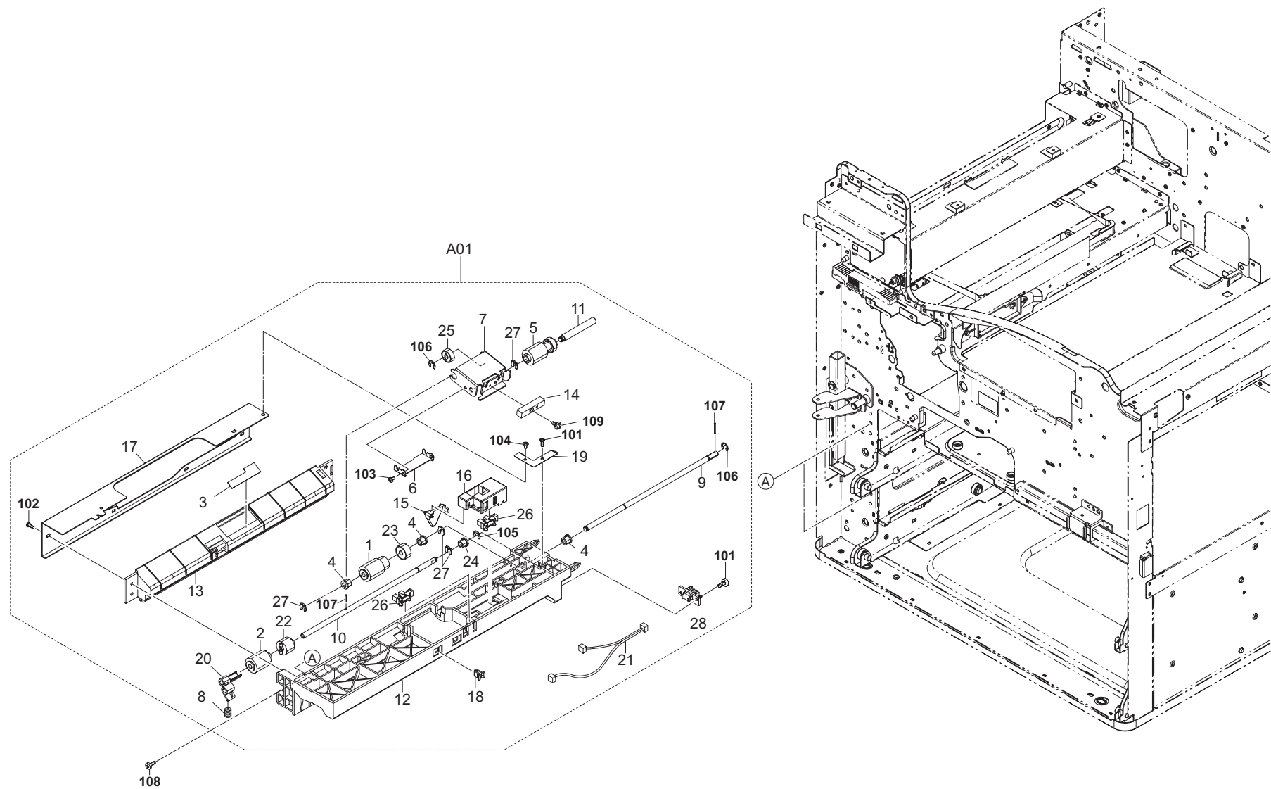
FIG. 4 Paper Feed-In I
