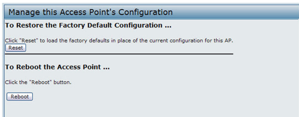
Figure 29: Maintenance
