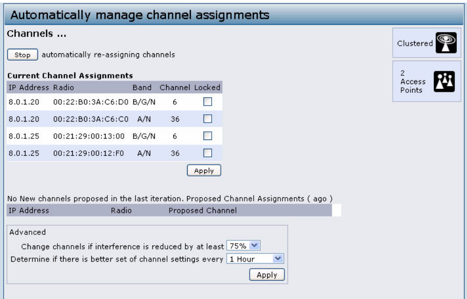
Figure 37: Channel Management
