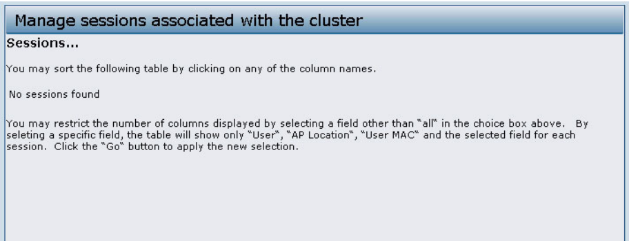
Figure 36: Session Management
