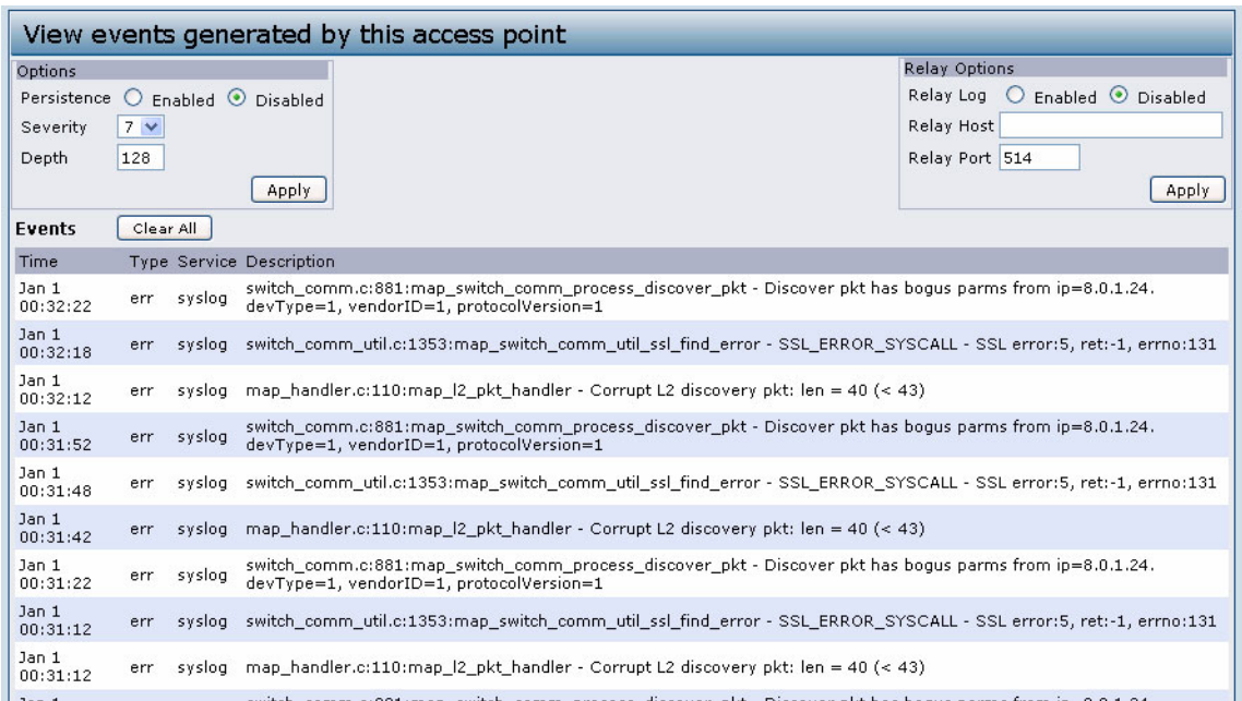
Figure 3: Viewing Events
