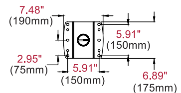
CEILING/FLOOR PLATE
