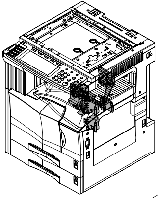
FIG. 16 DRIVING, COOLING SECTION I
