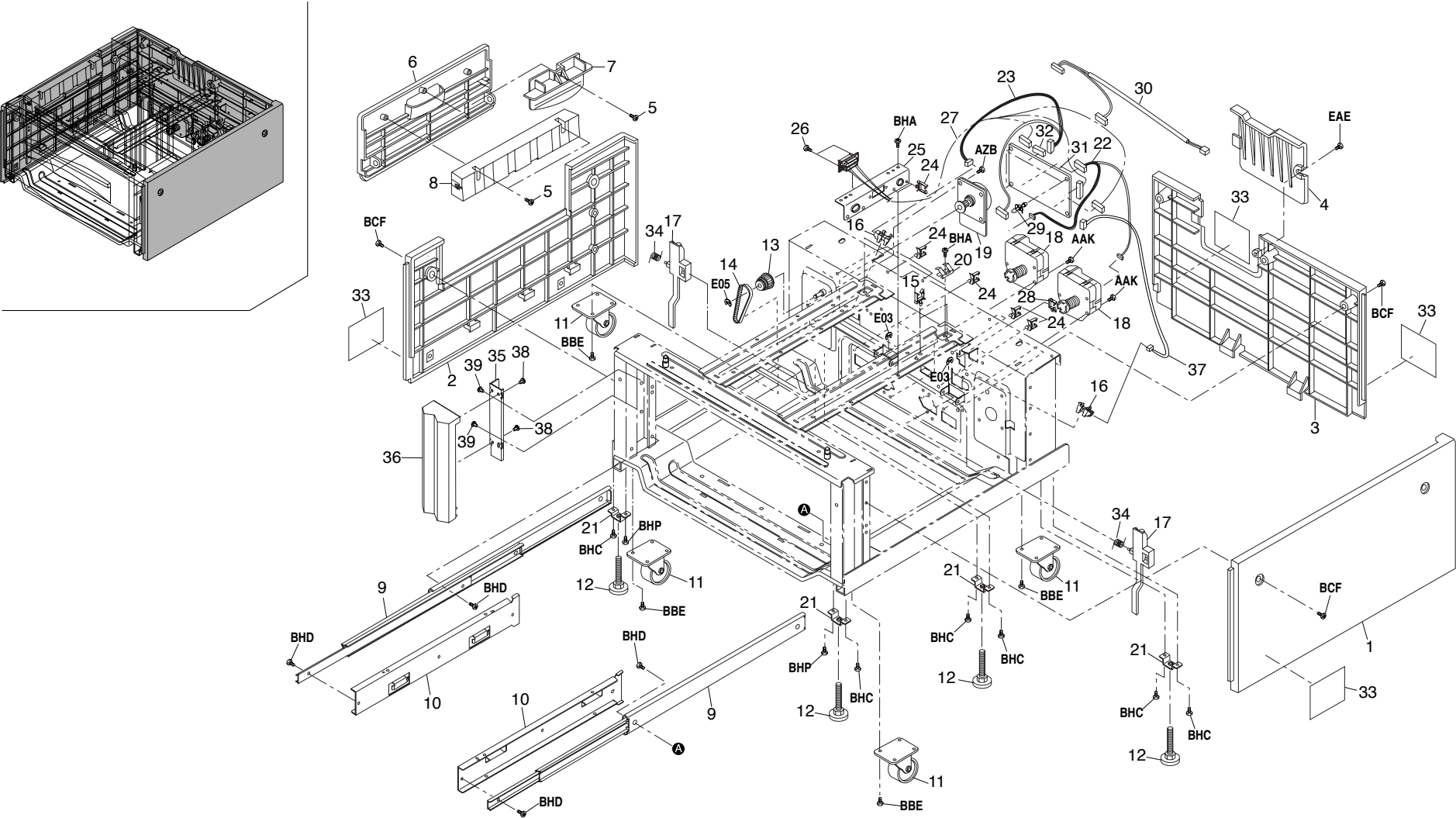
FIG. 1 EXTERIOR COVERS
