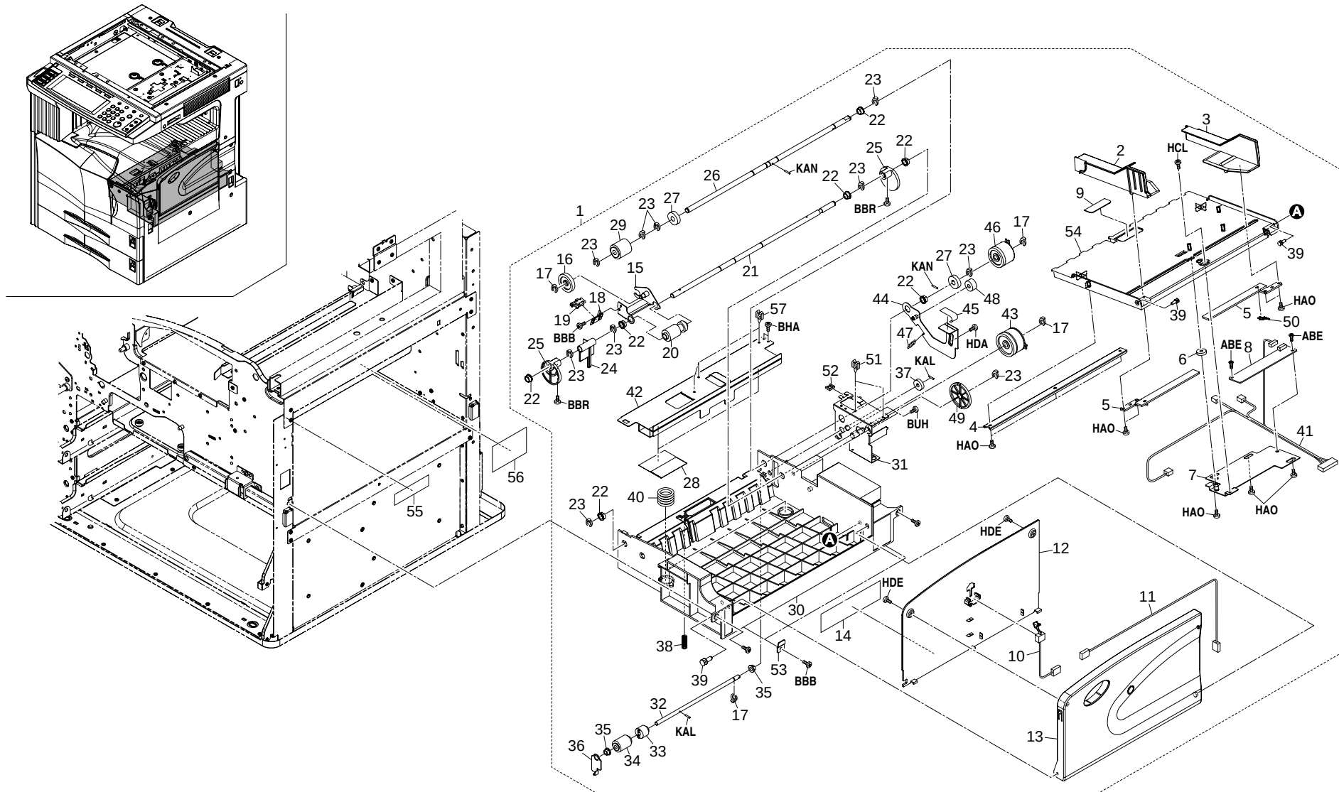
FIG. 10 BYPASS UNIT
