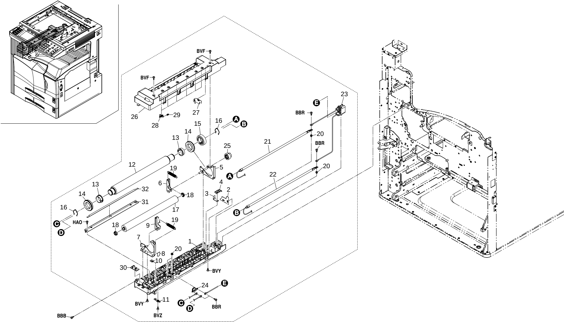
FIG. 14 FIXING SECTION
