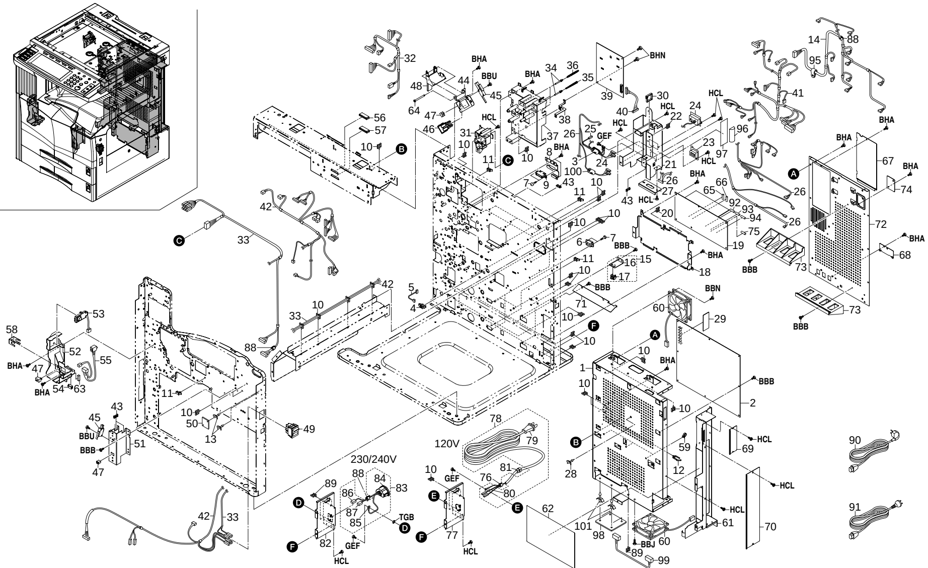
FIG. 18 ELECTRICAL COMPONENTS
