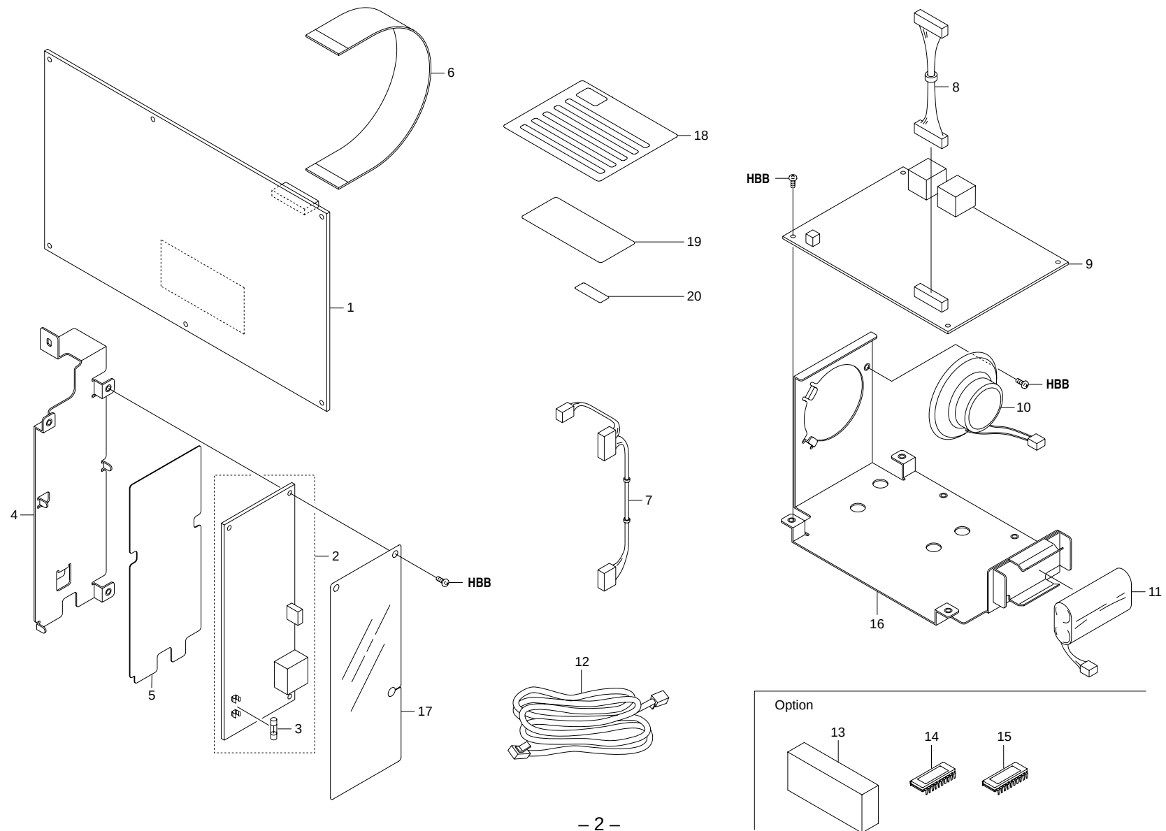
FIG. 1 FAX System(C)
