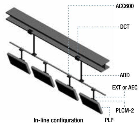
In-line configuration
