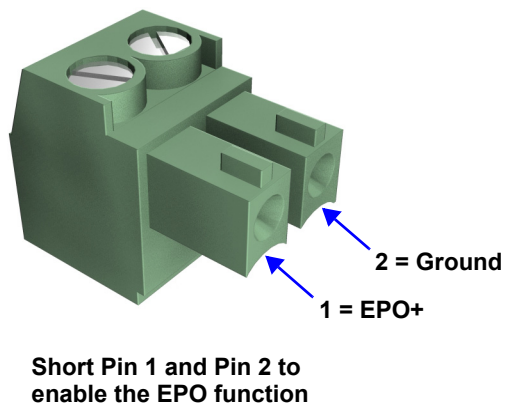
Figure 13 EPO connection for normally open operation
