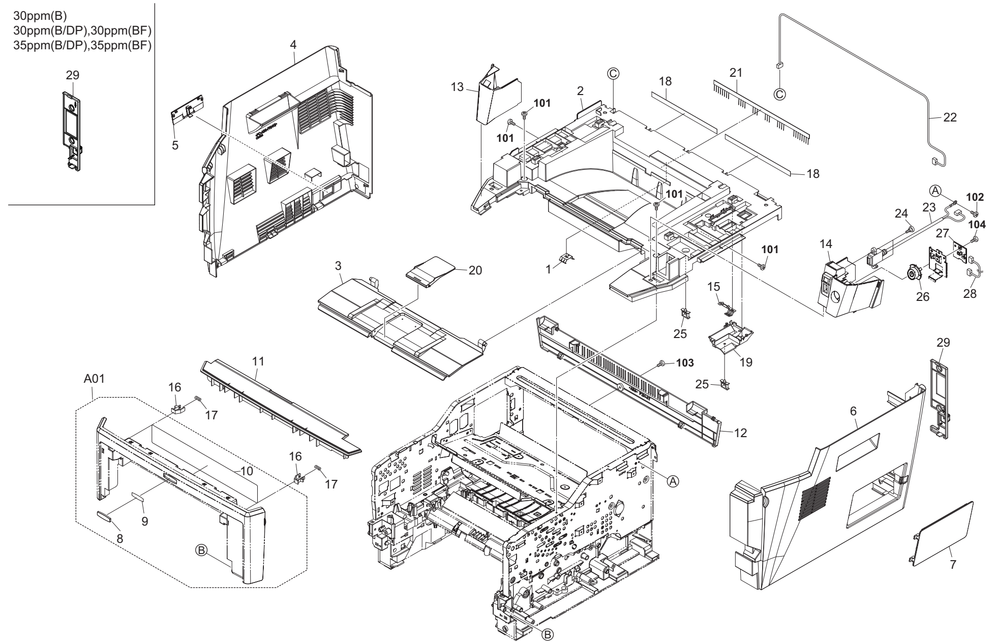
FIG. 1 Covers
