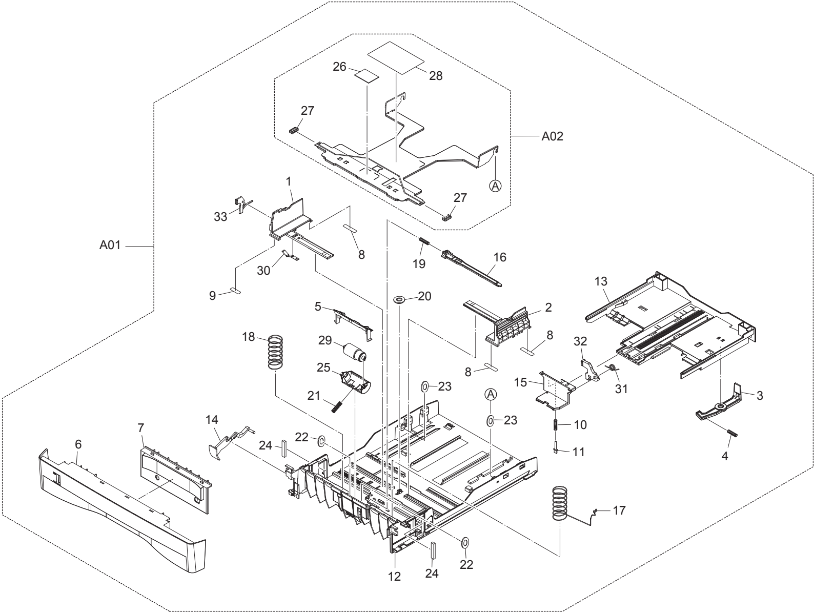
FIG. 3 Paper Cassette
