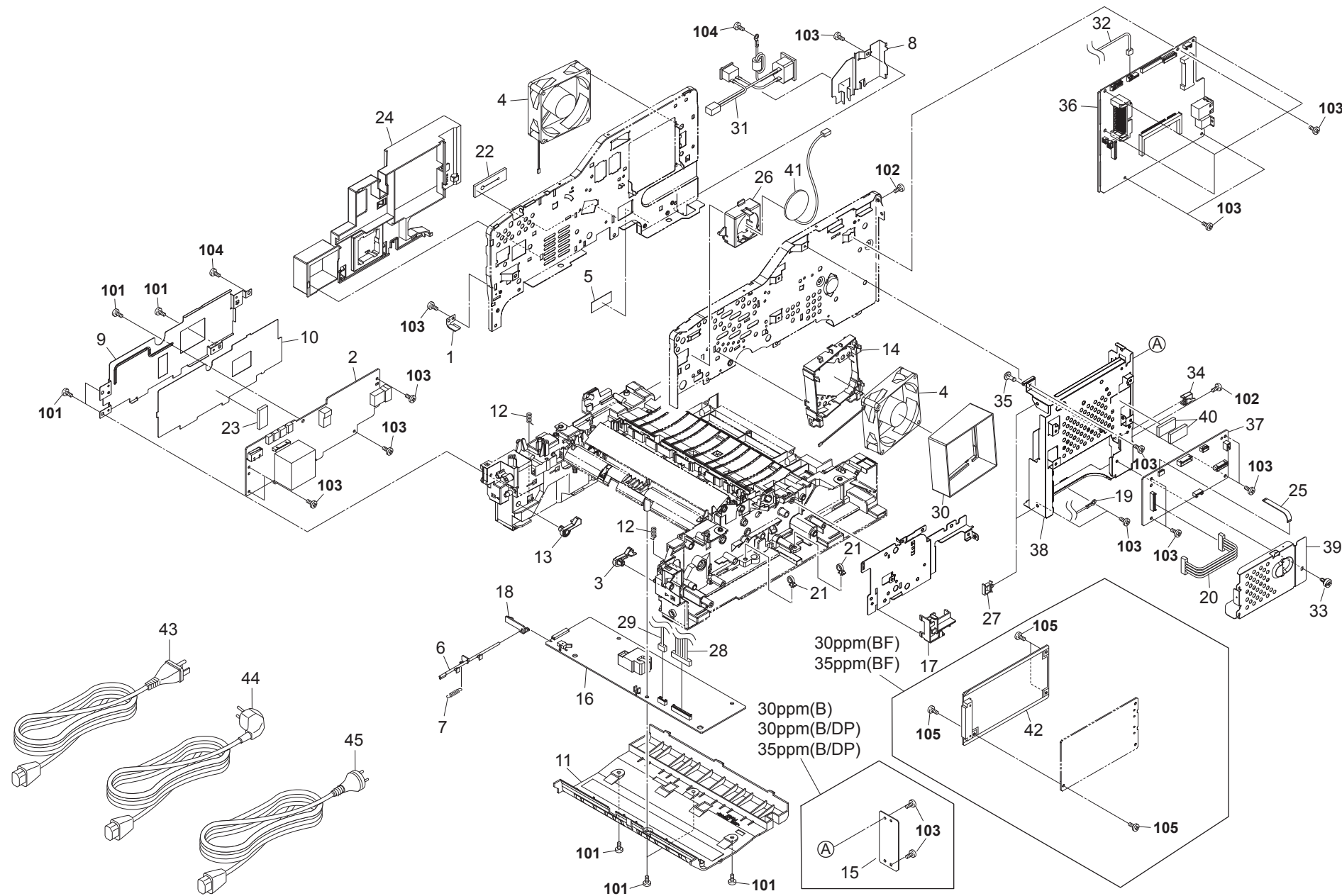
FIG. 12 Electrical Components(30ppm(B),30ppm(B/DP),30ppm(BF),35ppm(B/DP),35ppm(BF))
