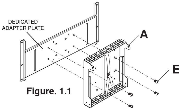
MOUNTING PATTERN FOR DEDICATED ADAPTER PLATES
