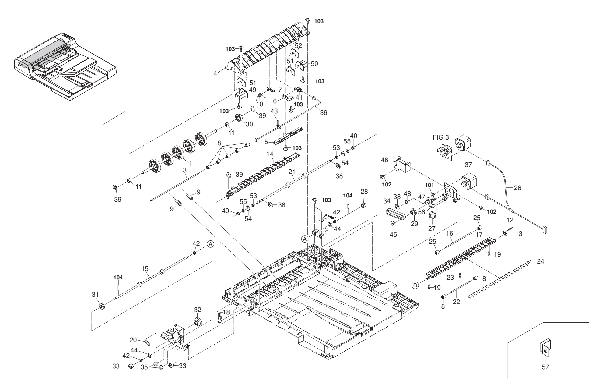
FIG. 4 Paper Conveying Section
