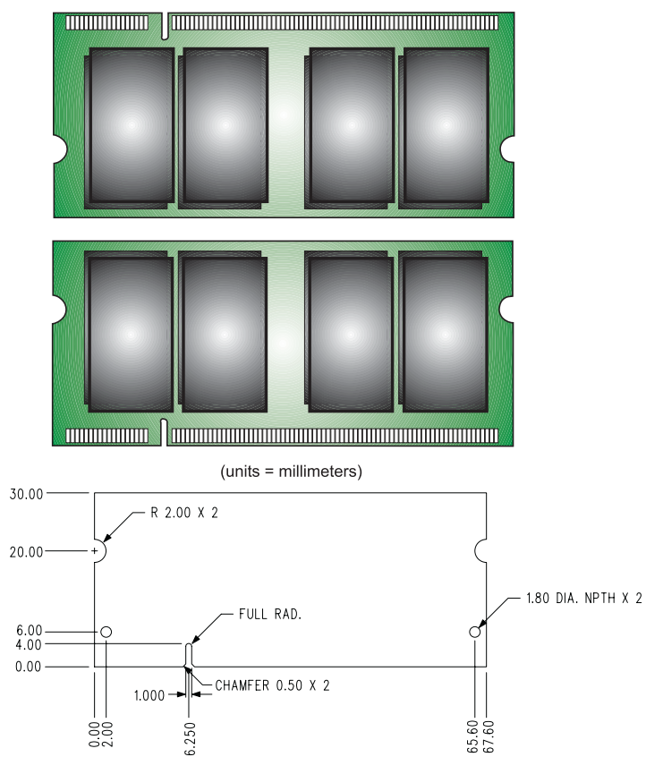
Figure 1: KVR533D2S4/2G 200-Pin SODIMM
