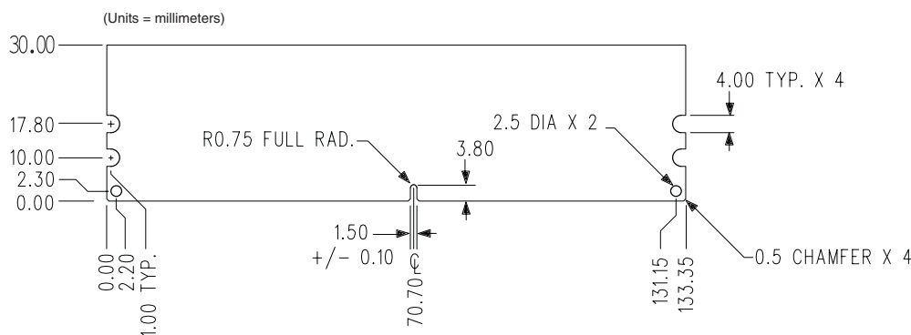
Figure 1: KVR800D2D8P5/1G 240-Pin DIMM
