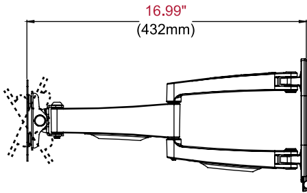
SIDE VIEW EXTENDED +/-35° TILT
