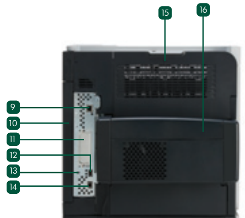
Partial rear view I/O panel
