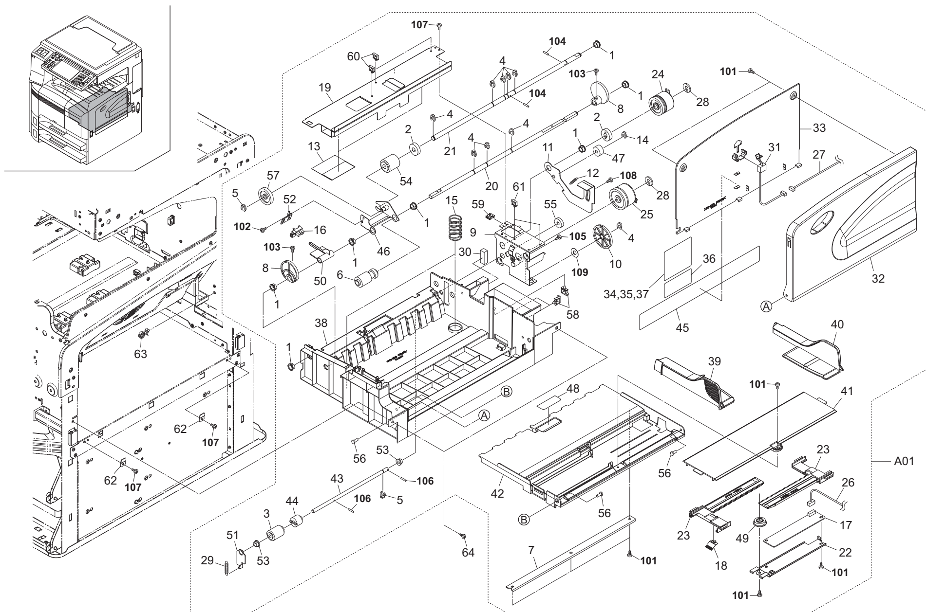
FIG. 6 Paper Feed Section 3
