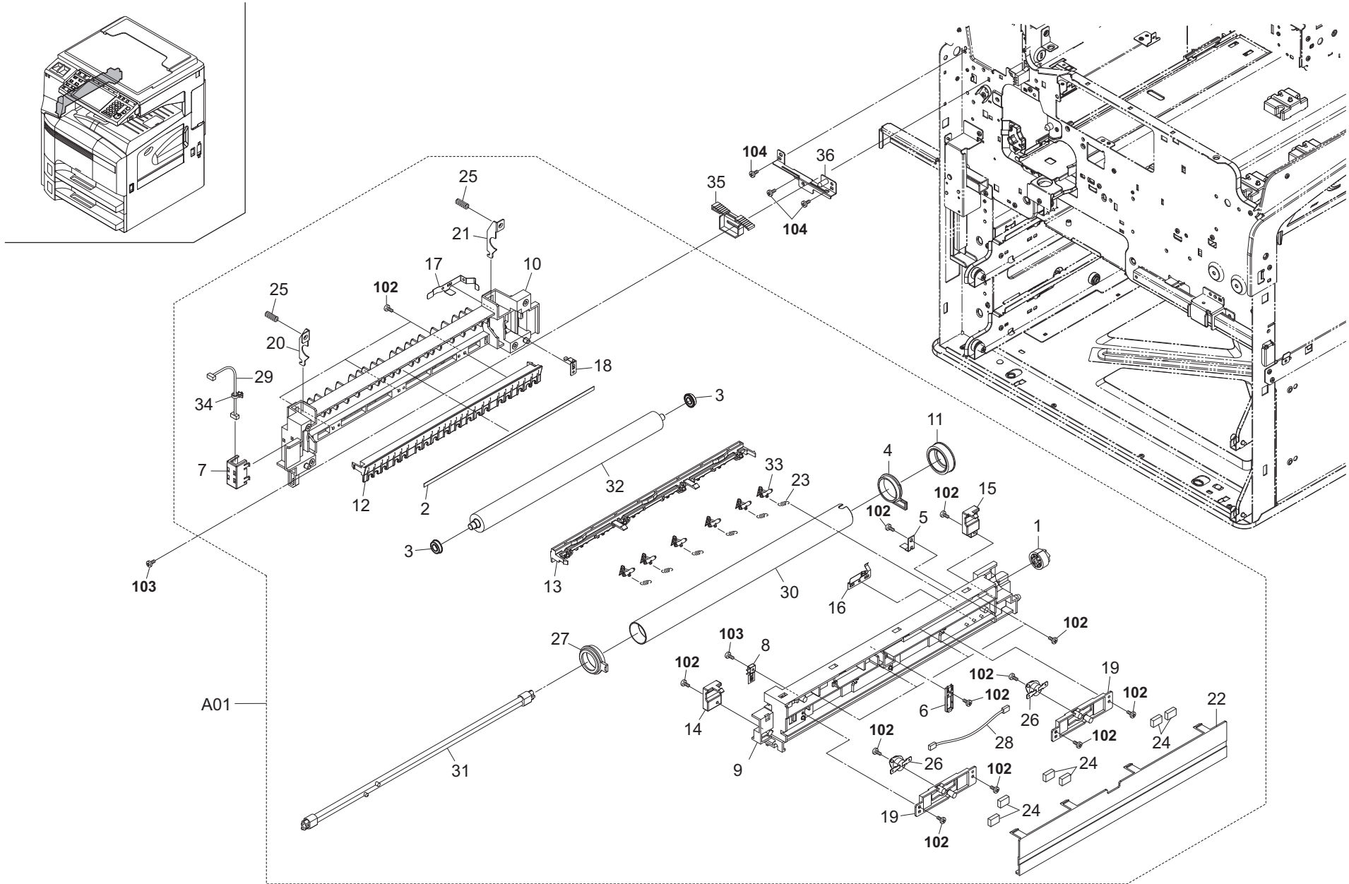
FIG. 14 Fuser Section 2K5
