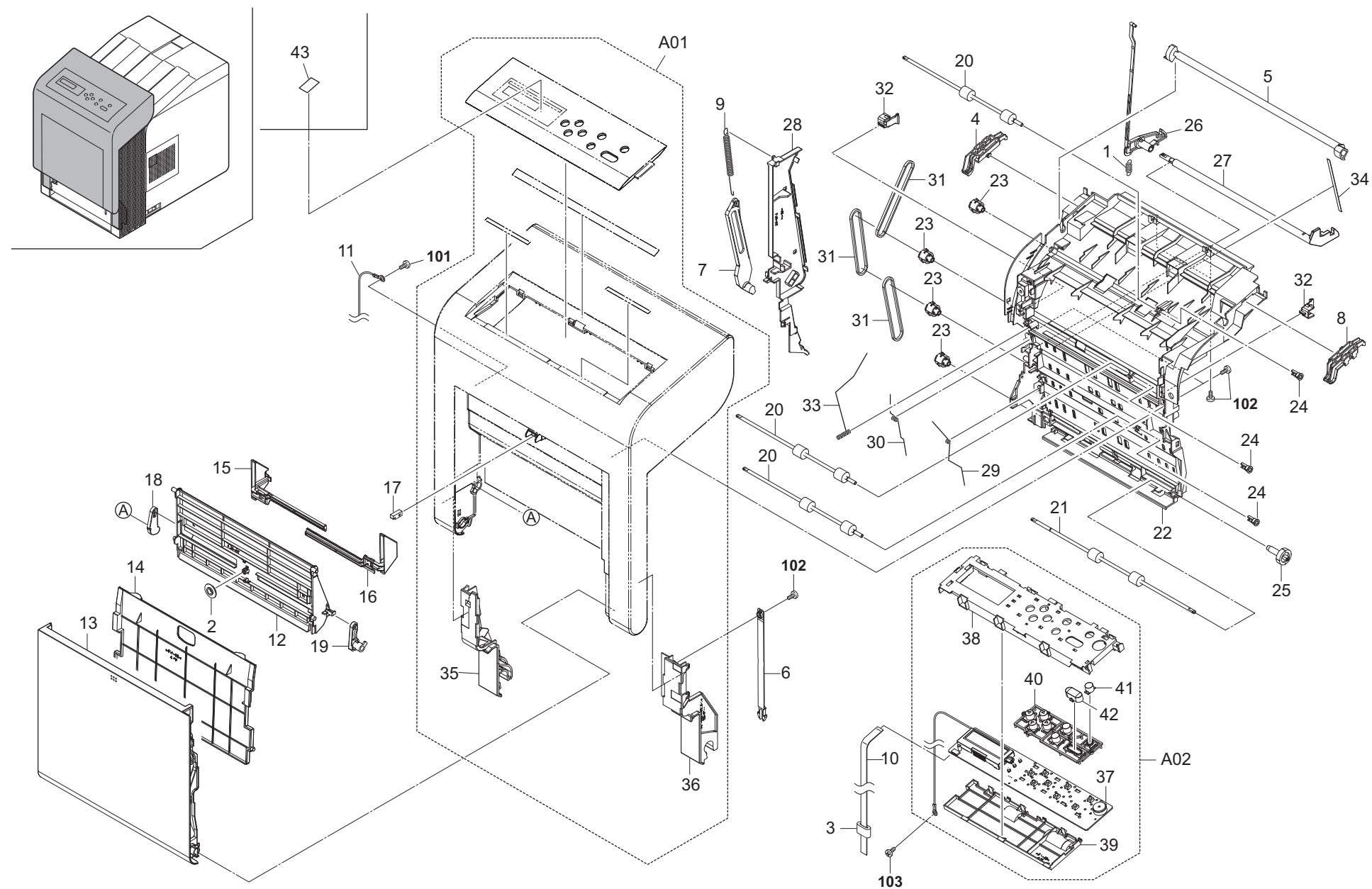
FIG. 2 Covers 2
