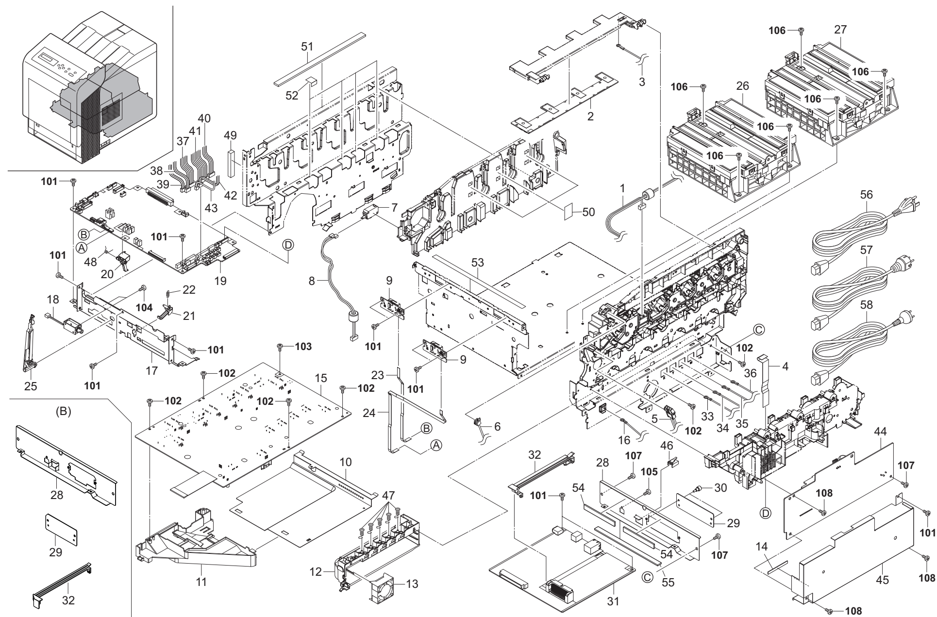
FIG. 14 Electrical Components
