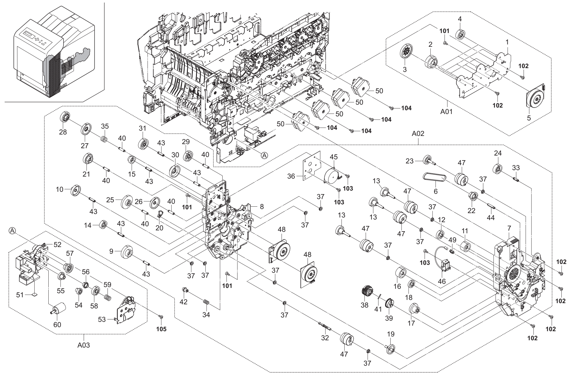
FIG. 12 Drive Section
