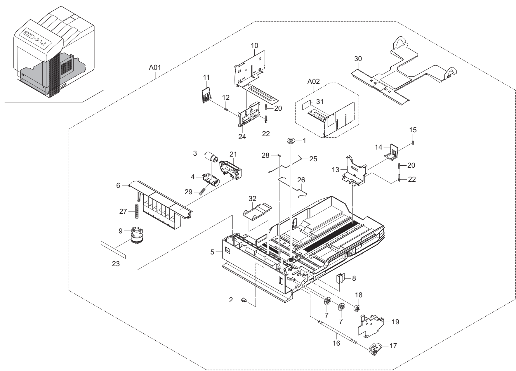
FIG. 5 Paper Cassette
