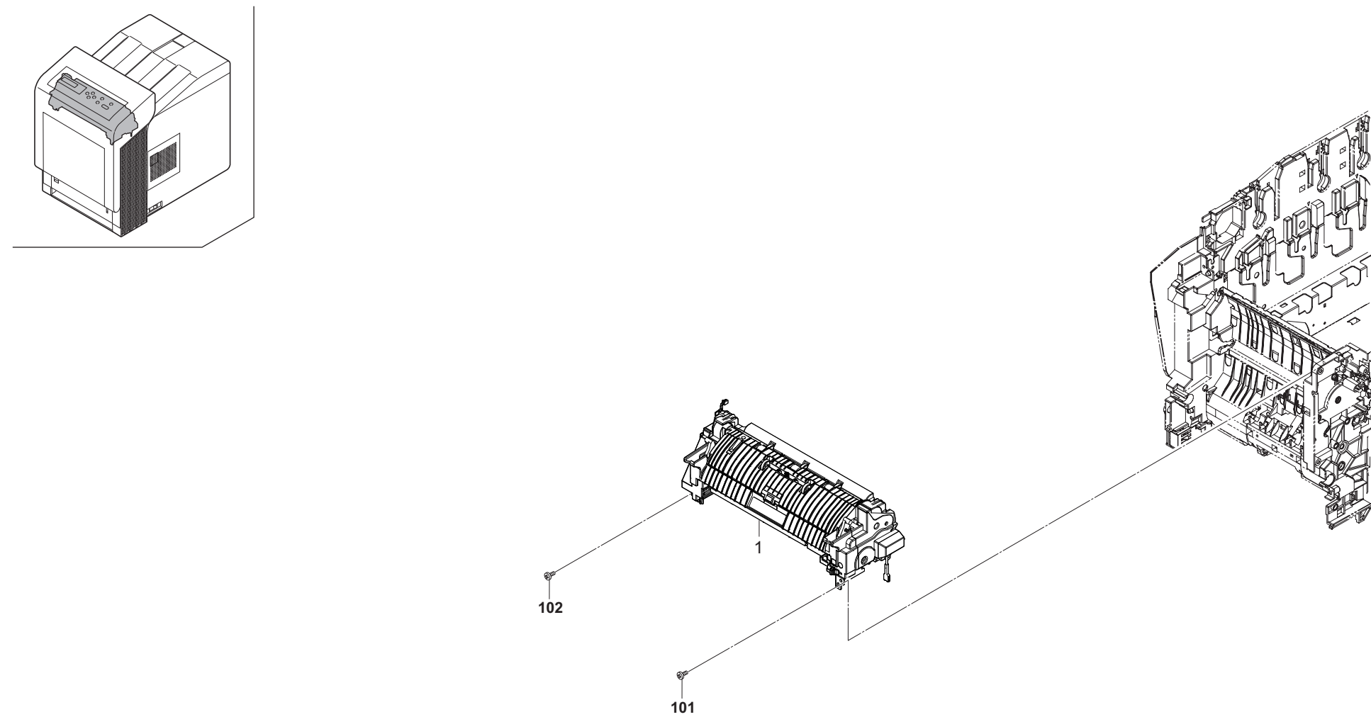
FIG. 11 Fuser Section
