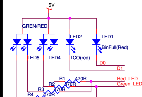
Design D+ LED PCBA
