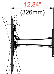
SIDE VIEW EXTENDED +15°/-5° TILT
