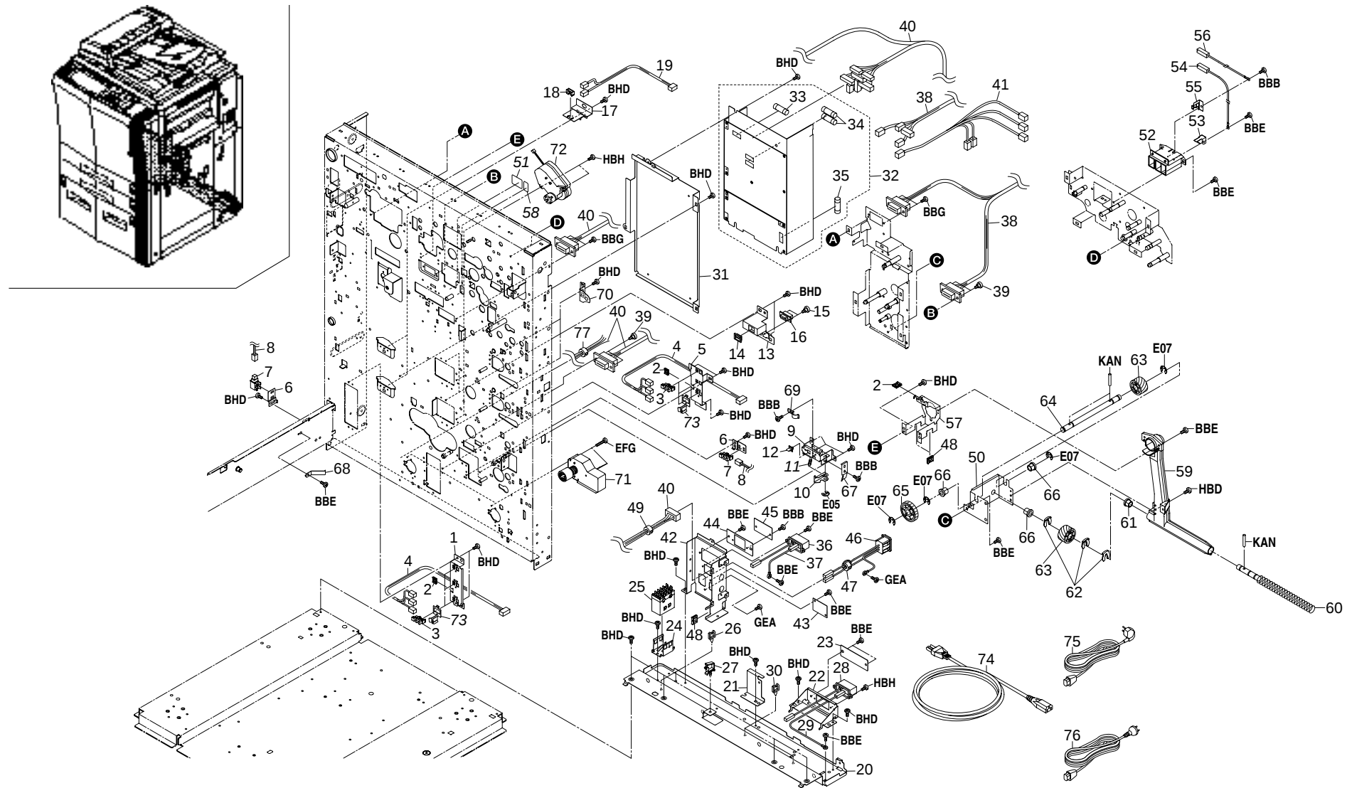
FIG. 39 ELECTRICAL SECTION I
