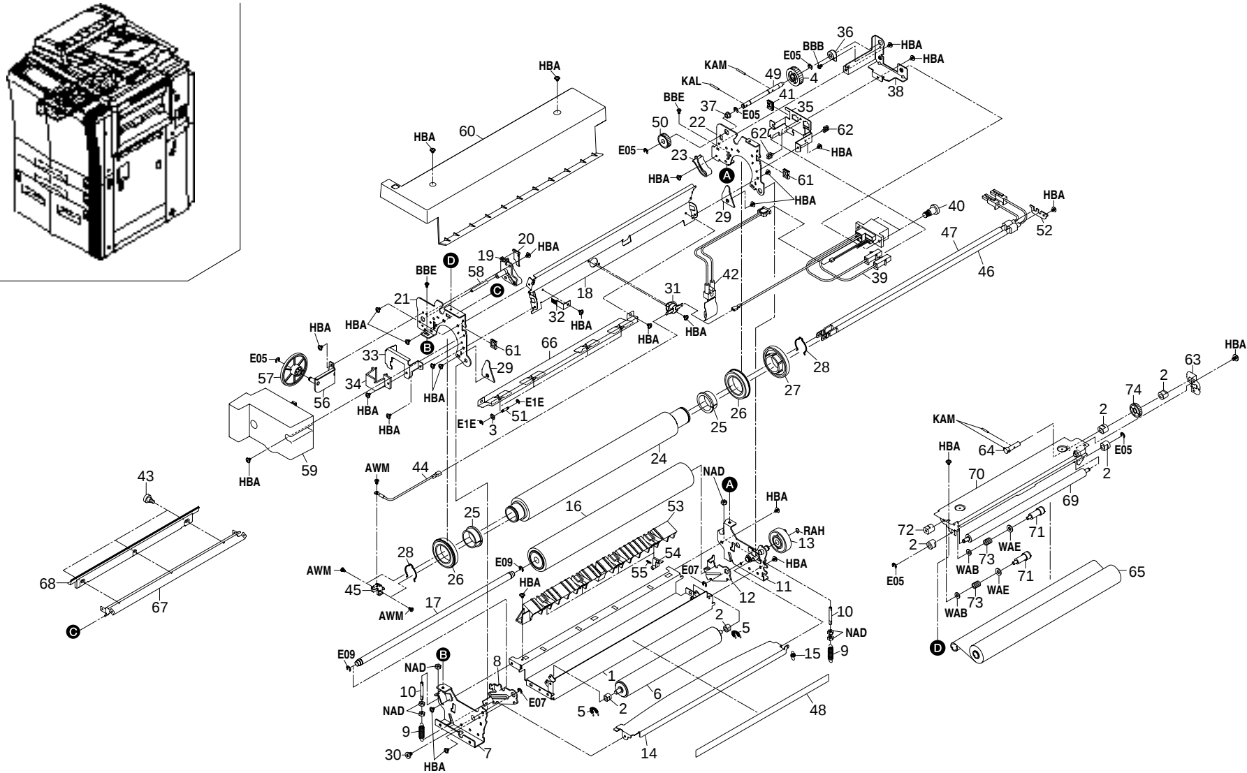
FIG. 19 FIXING SECTION
