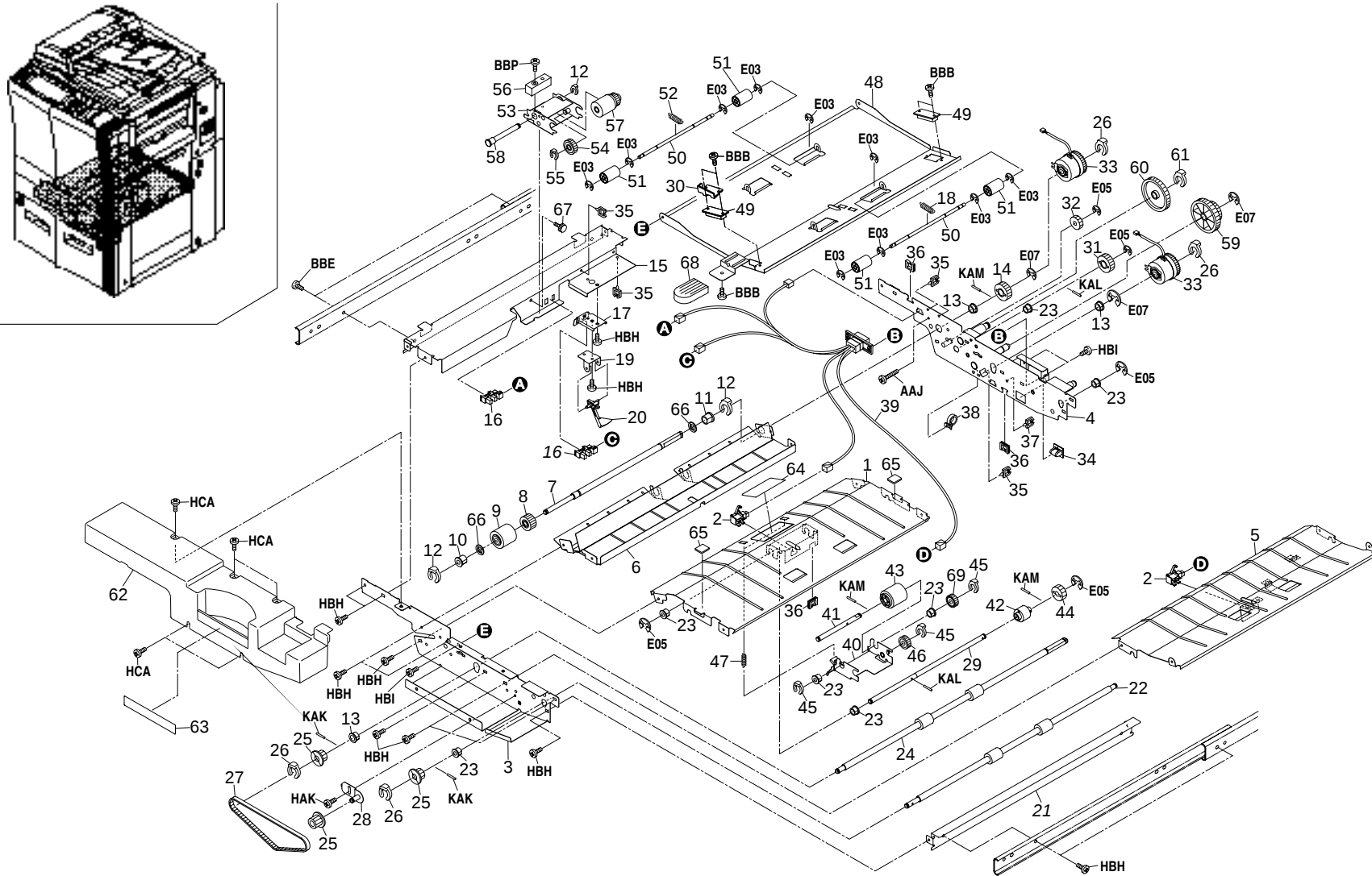
FIG. 6 DECK CONVEYING SECTION
