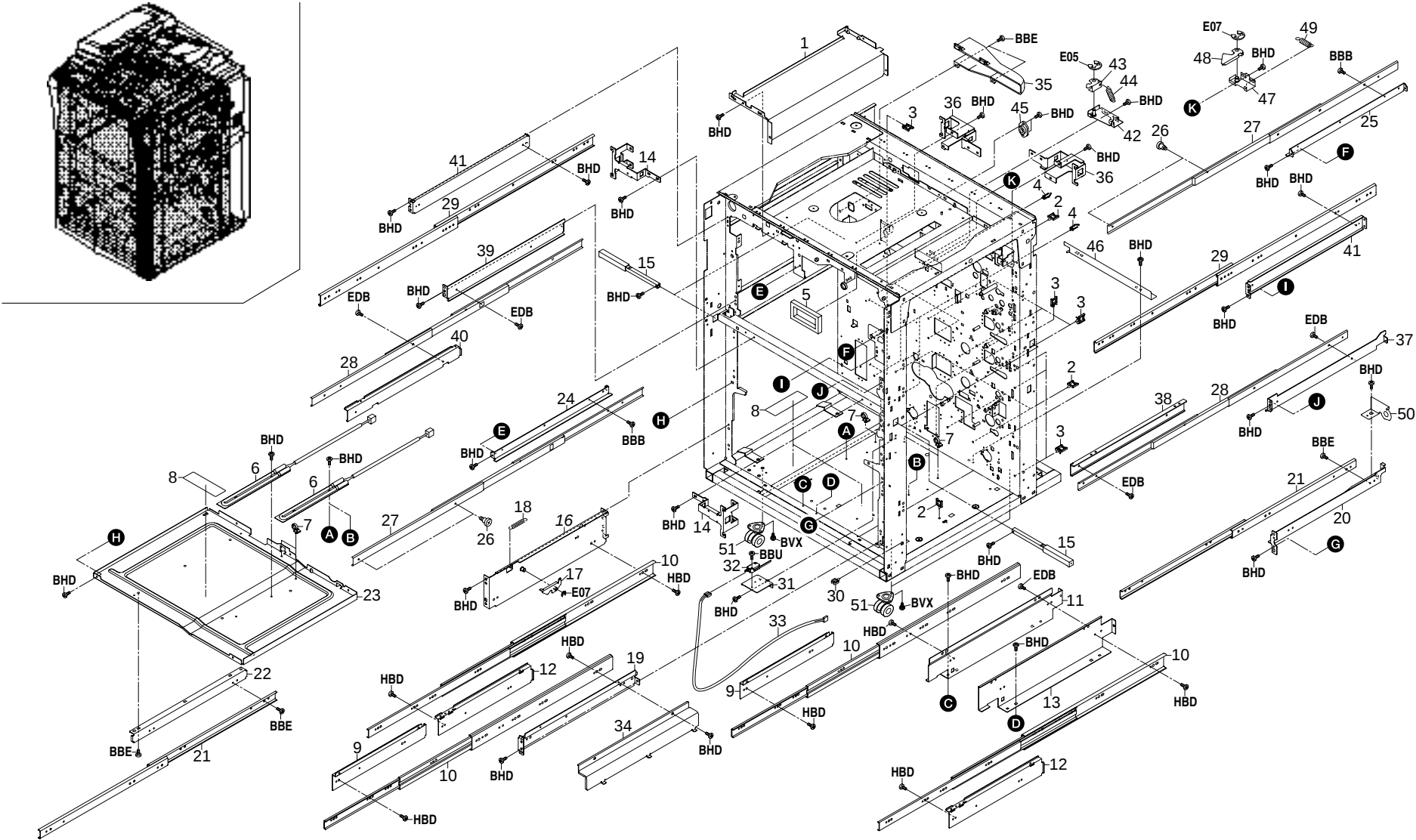
FIG. 2 FRAME SECTION
