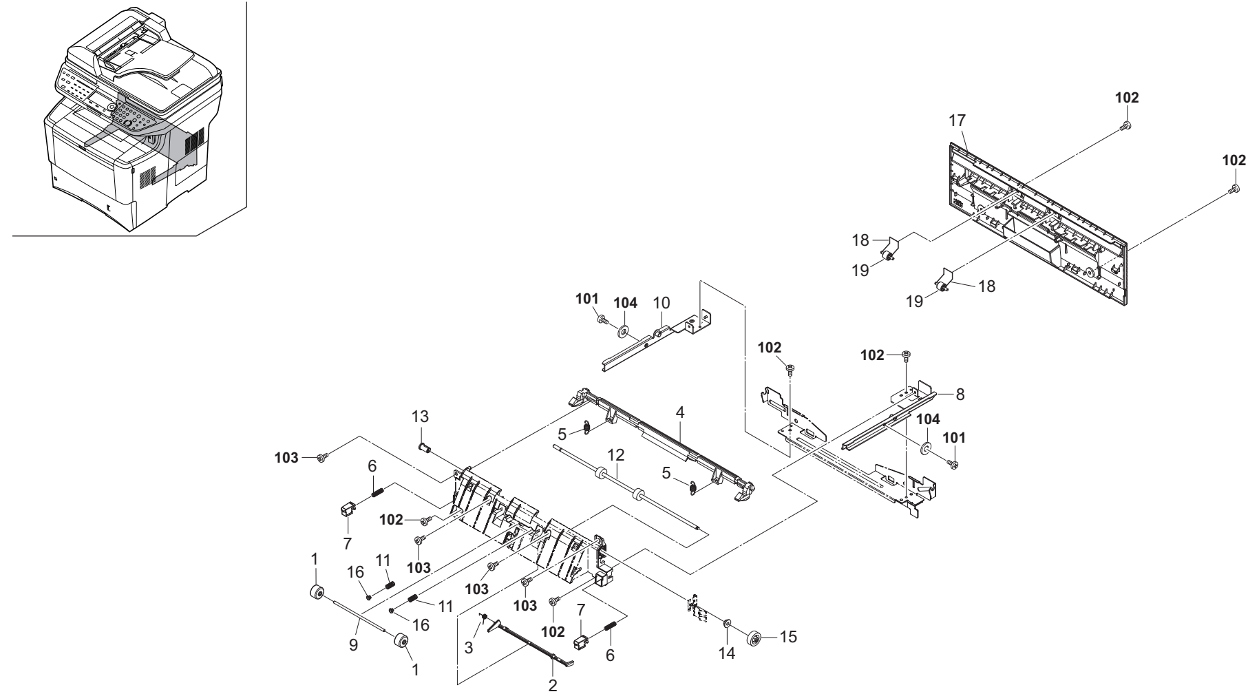
FIG. 13 Fuser Section 2
