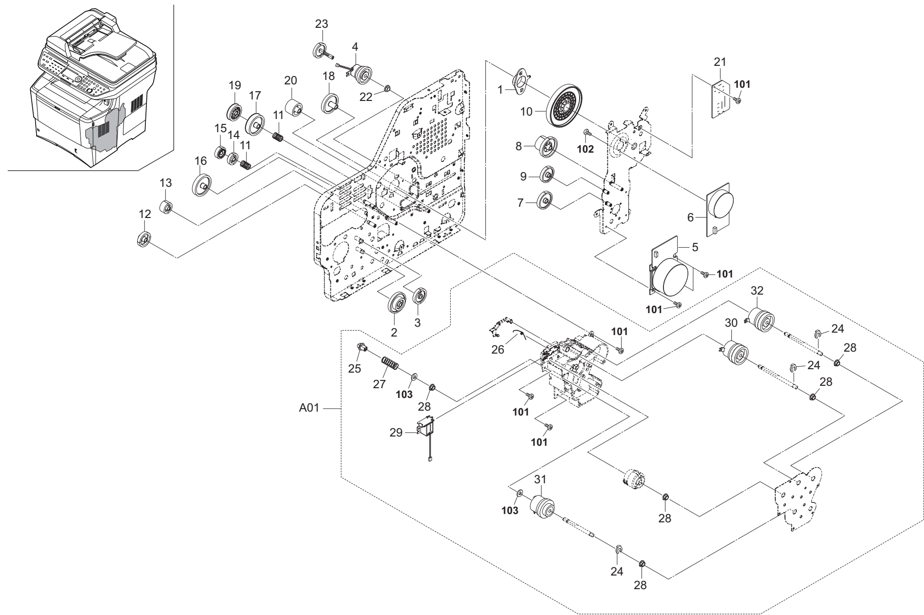
FIG. 14 Drive Section
