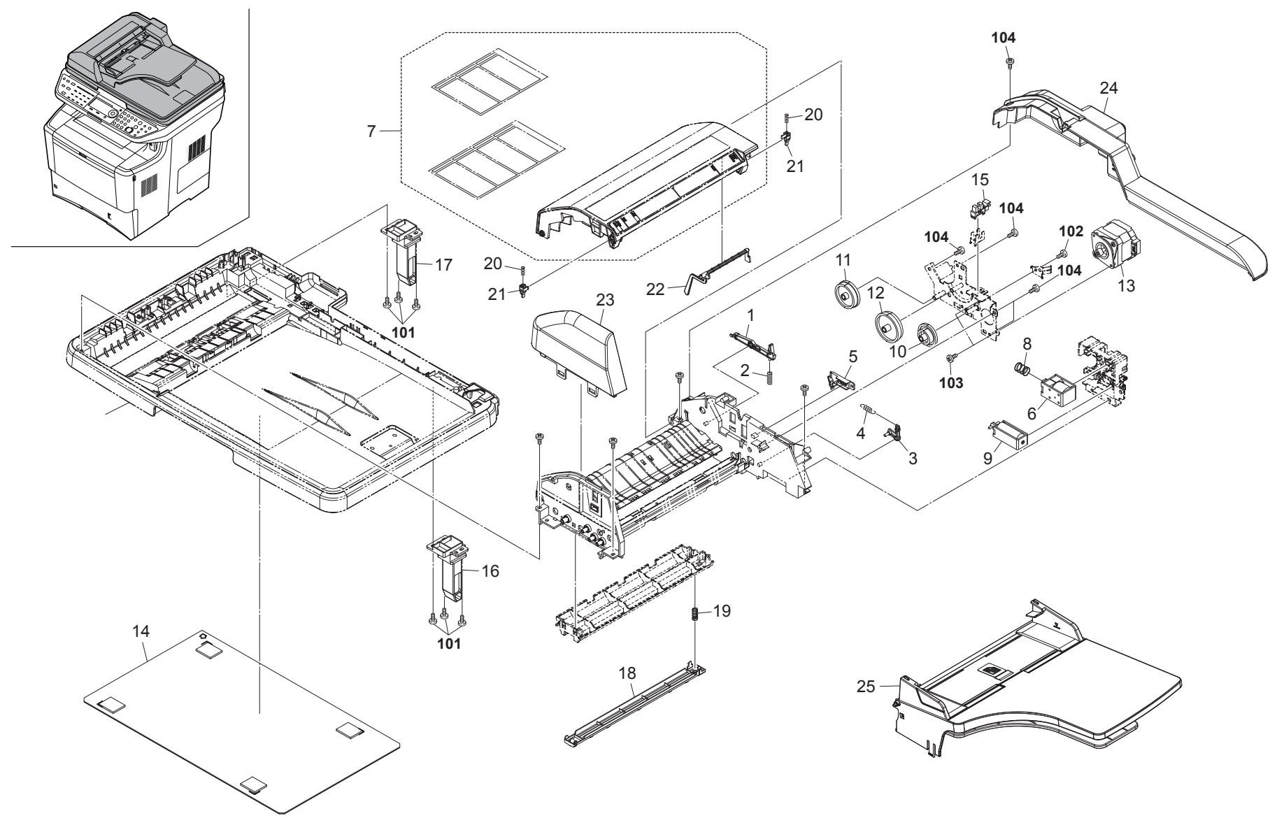
FIG. 19 Document Processor 2
