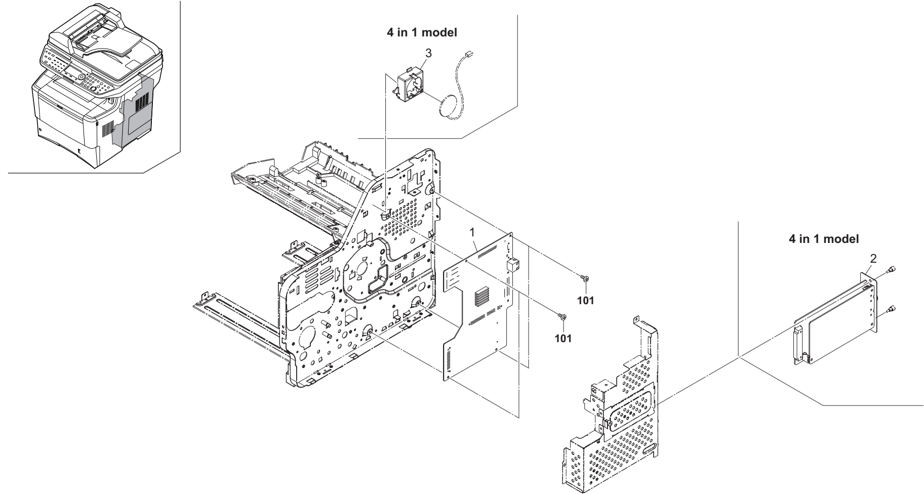
FIG. 16 Electrical Components
