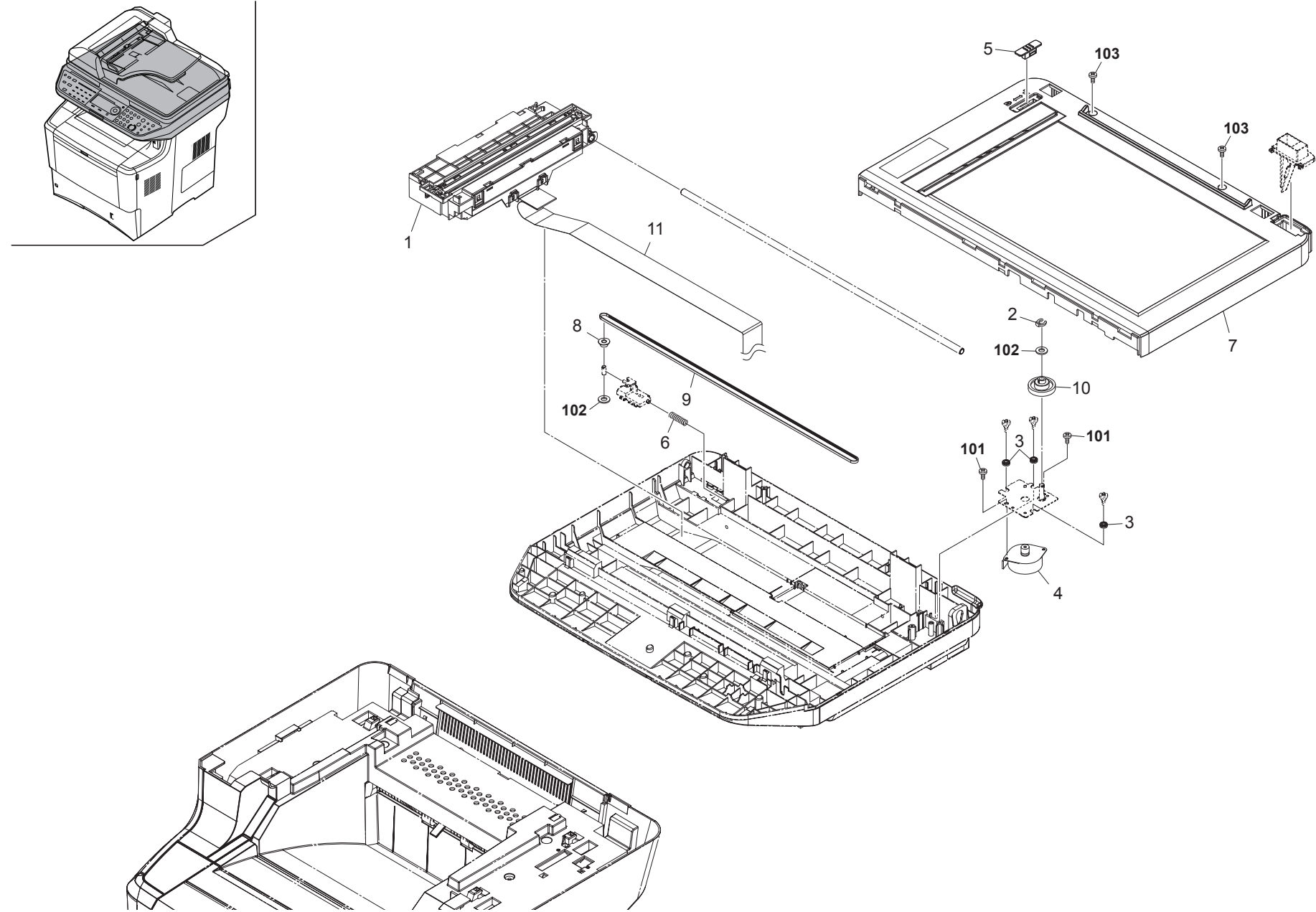
FIG. 9 Scanner Section
