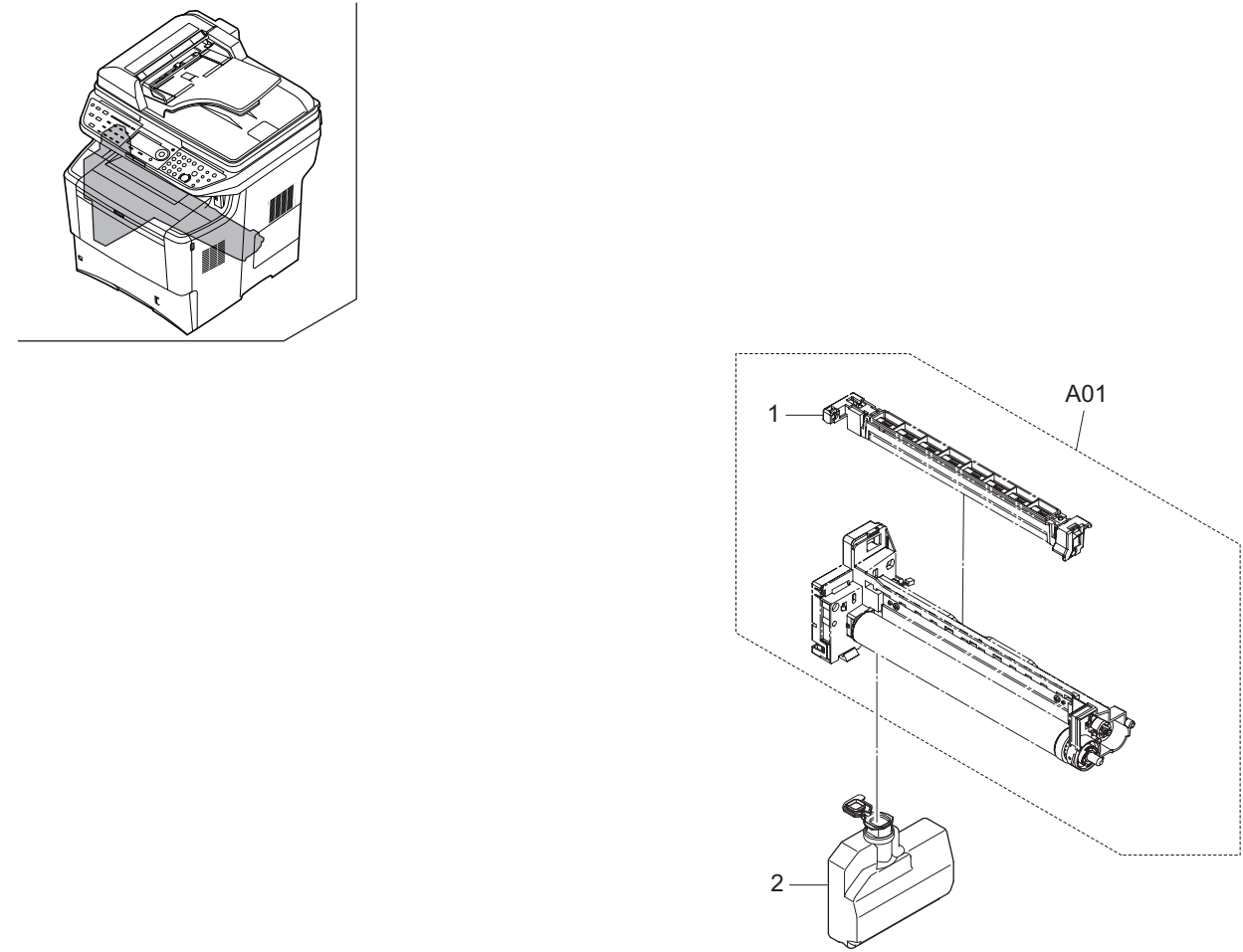
FIG. 10 Image Formation Section
