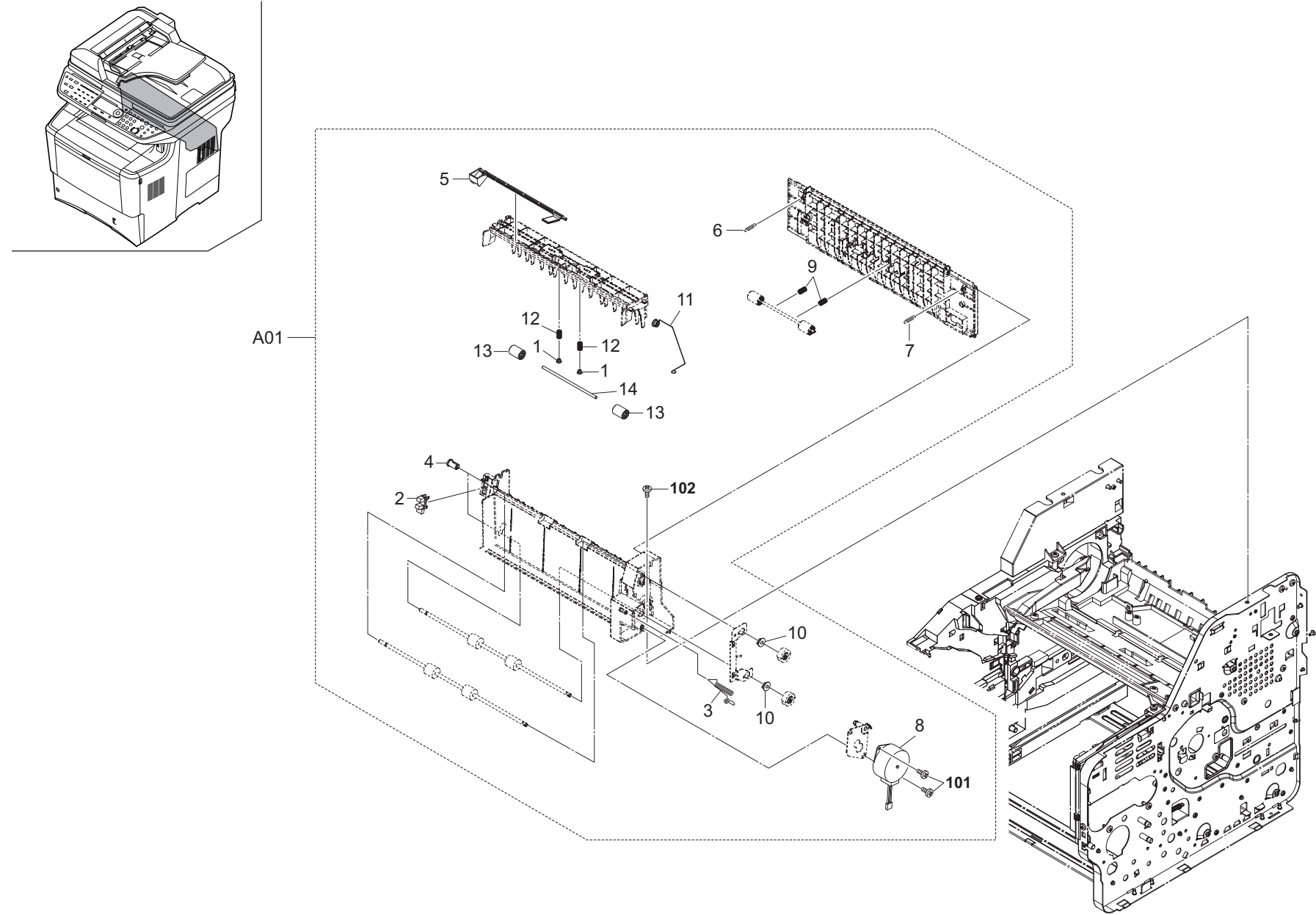
FIG. 15 Exit Section
