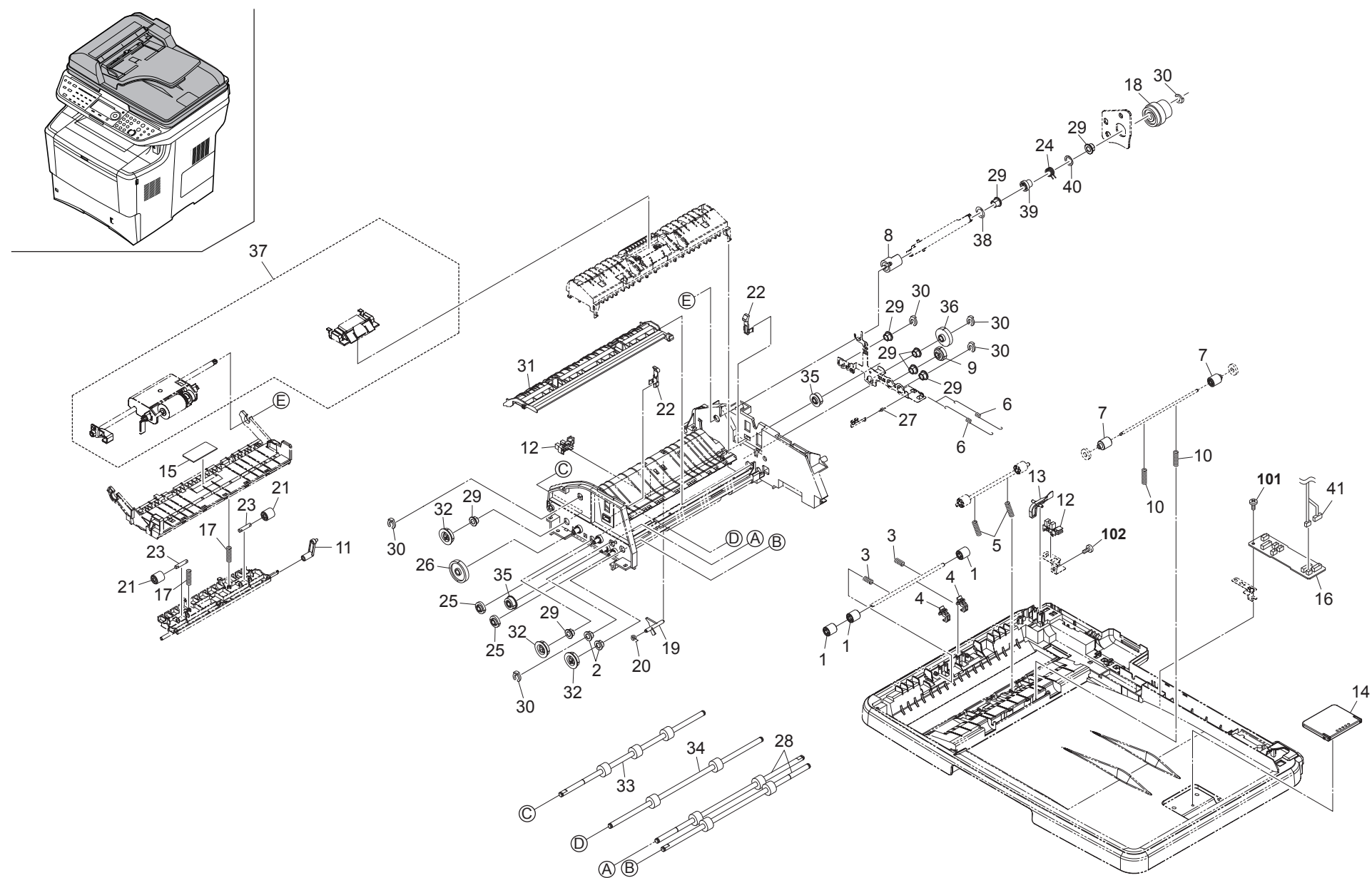
FIG. 18 Document Processor 1
