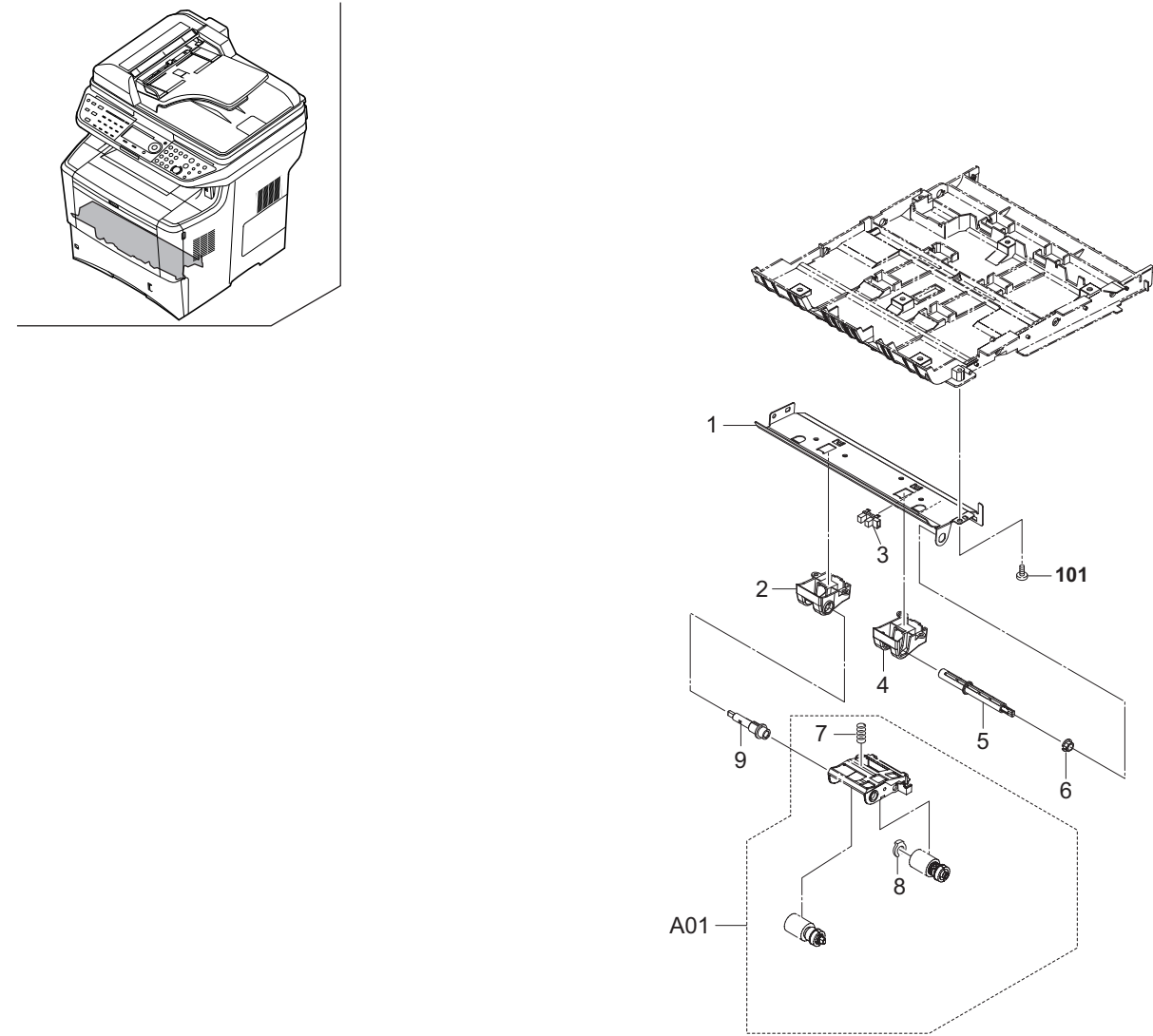
FIG. 7 Paper Feed Section 3
