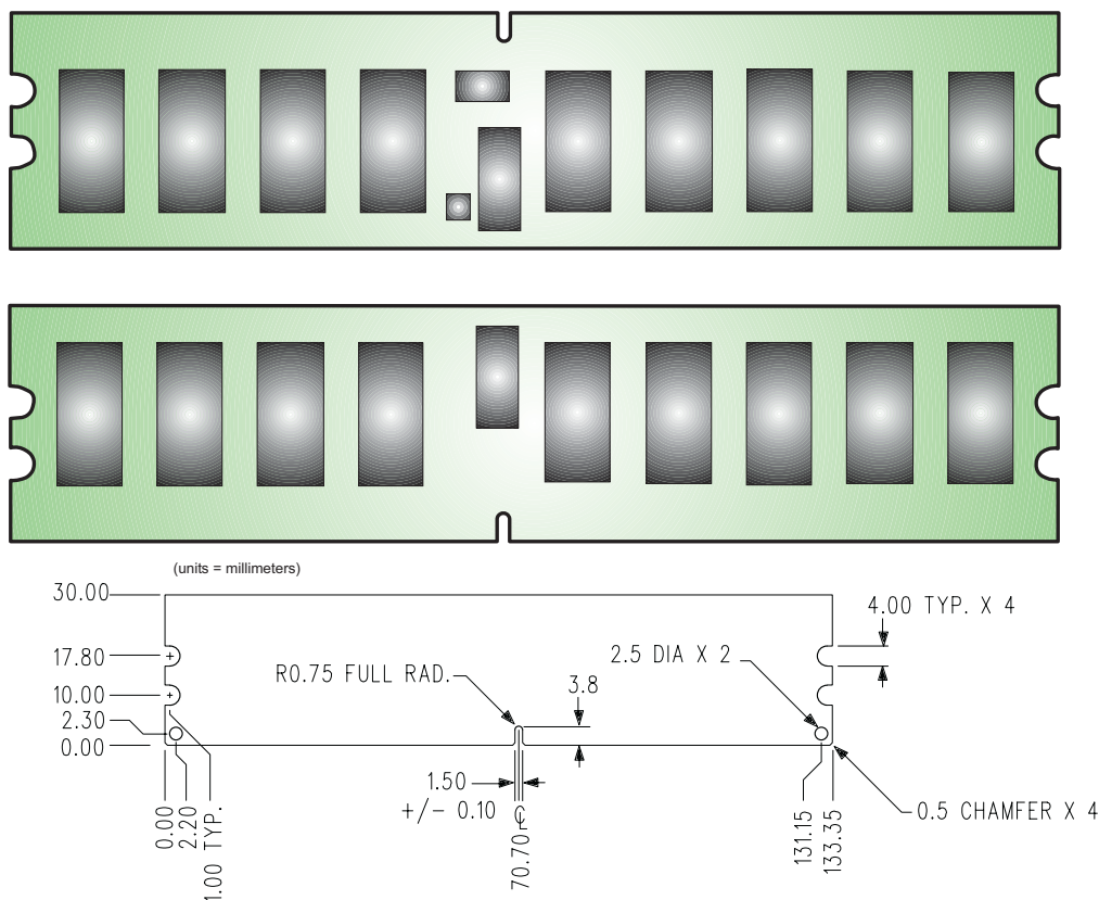
Figure 1: KVR667D2S4P5/4G 240-Pin DIMM
