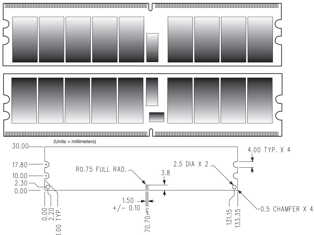
Figure 1: KVR533D2S4R4K2/4G 240-Pin DIMM
