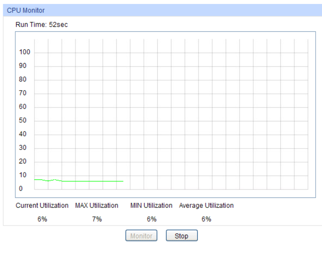
Figure 15-1 CPU Monitor
