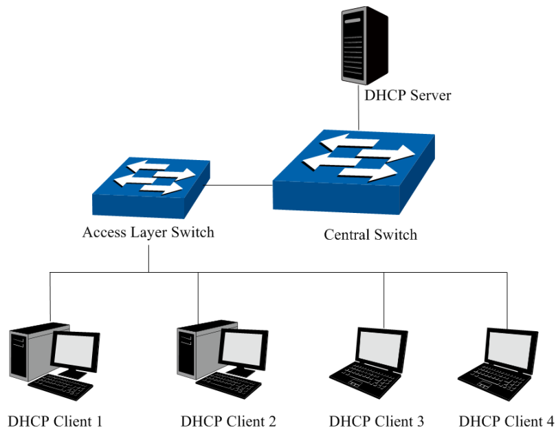
Figure 5-17 Network diagram of DHCP
