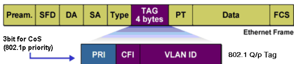
Figure 9-2 802.1Q frame
