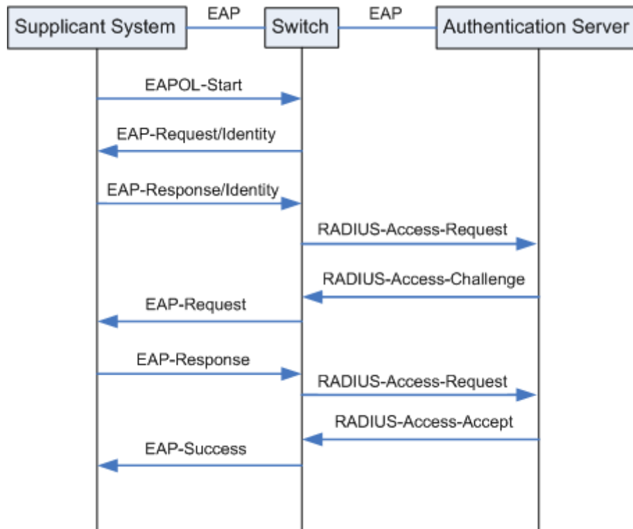
Figure 11-2 EAP-MD5 Authentication Procedure
