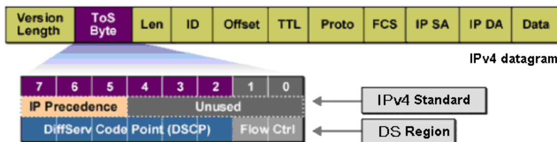
Figure 9-3 IP datagram
