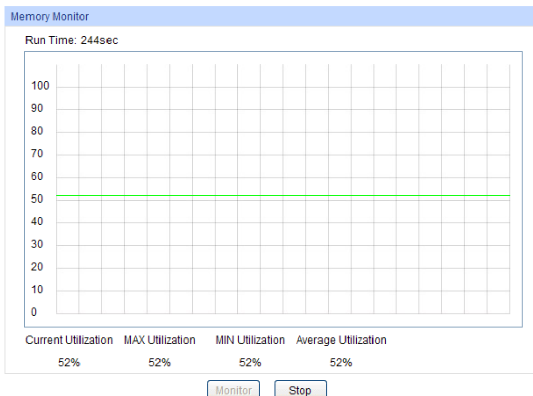
Figure 15-2 Memory Monitor
