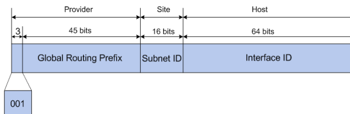
Figure 4-8 Global Unicast Address Format
