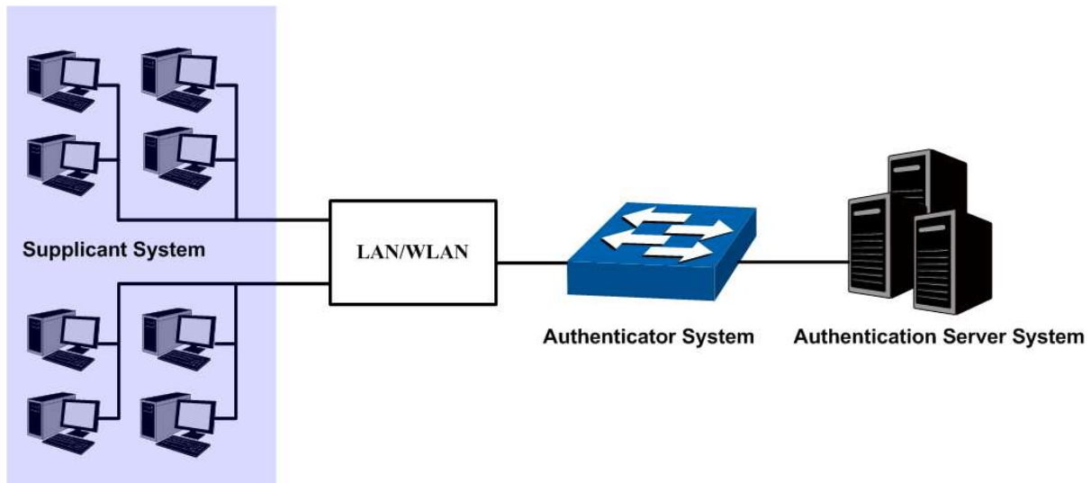
Figure 11-1 Architecture of 802.1X authentication
