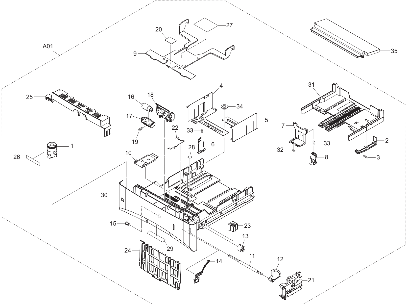
FIG. 4 Paper Cassette (FS-4020DN/3920DN)
