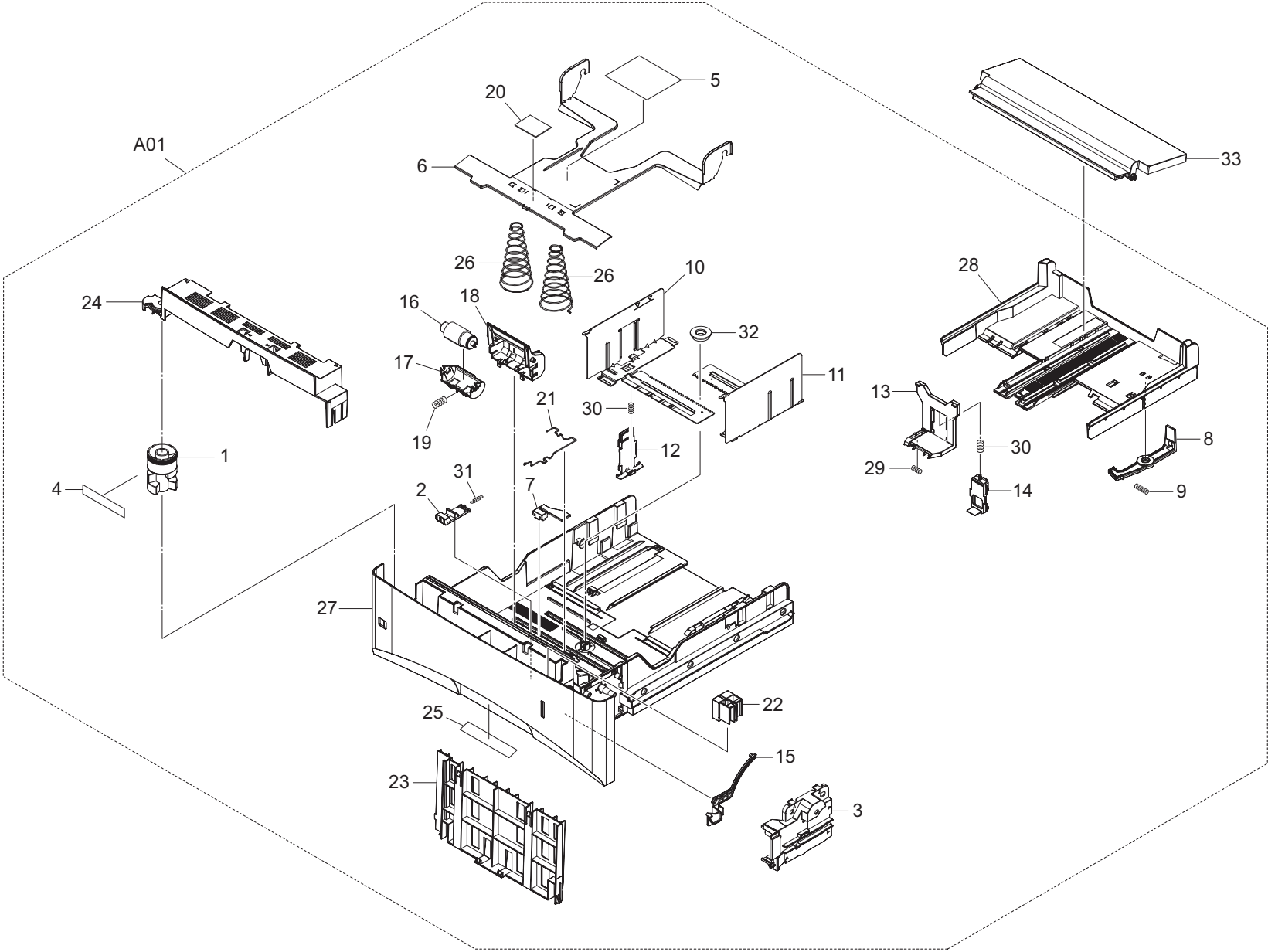
FIG. 4 Paper Cassette (FS-2020D)
