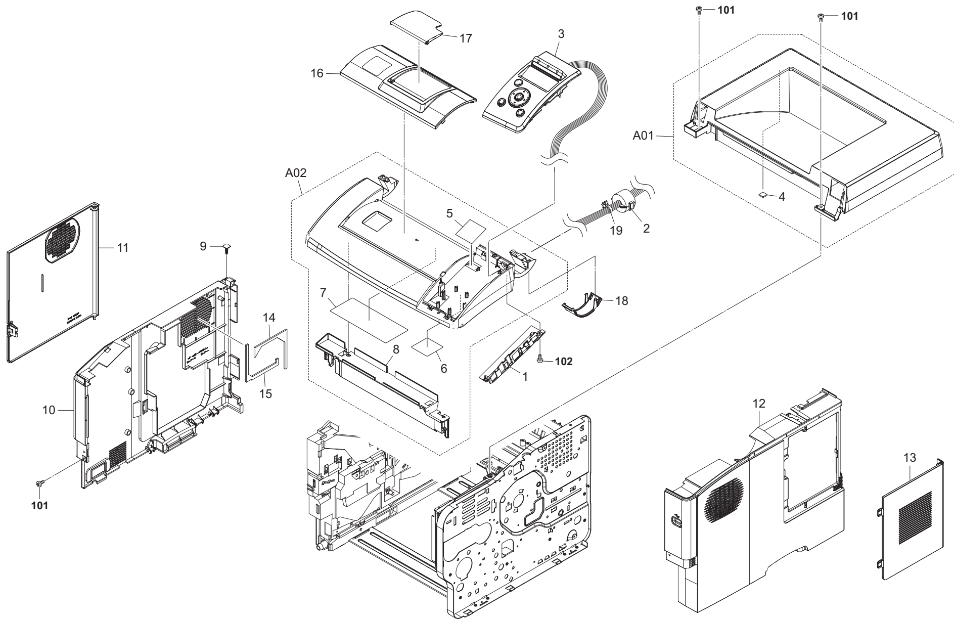
FIG. 1 Covers (FS-4020DN/3920DN)
