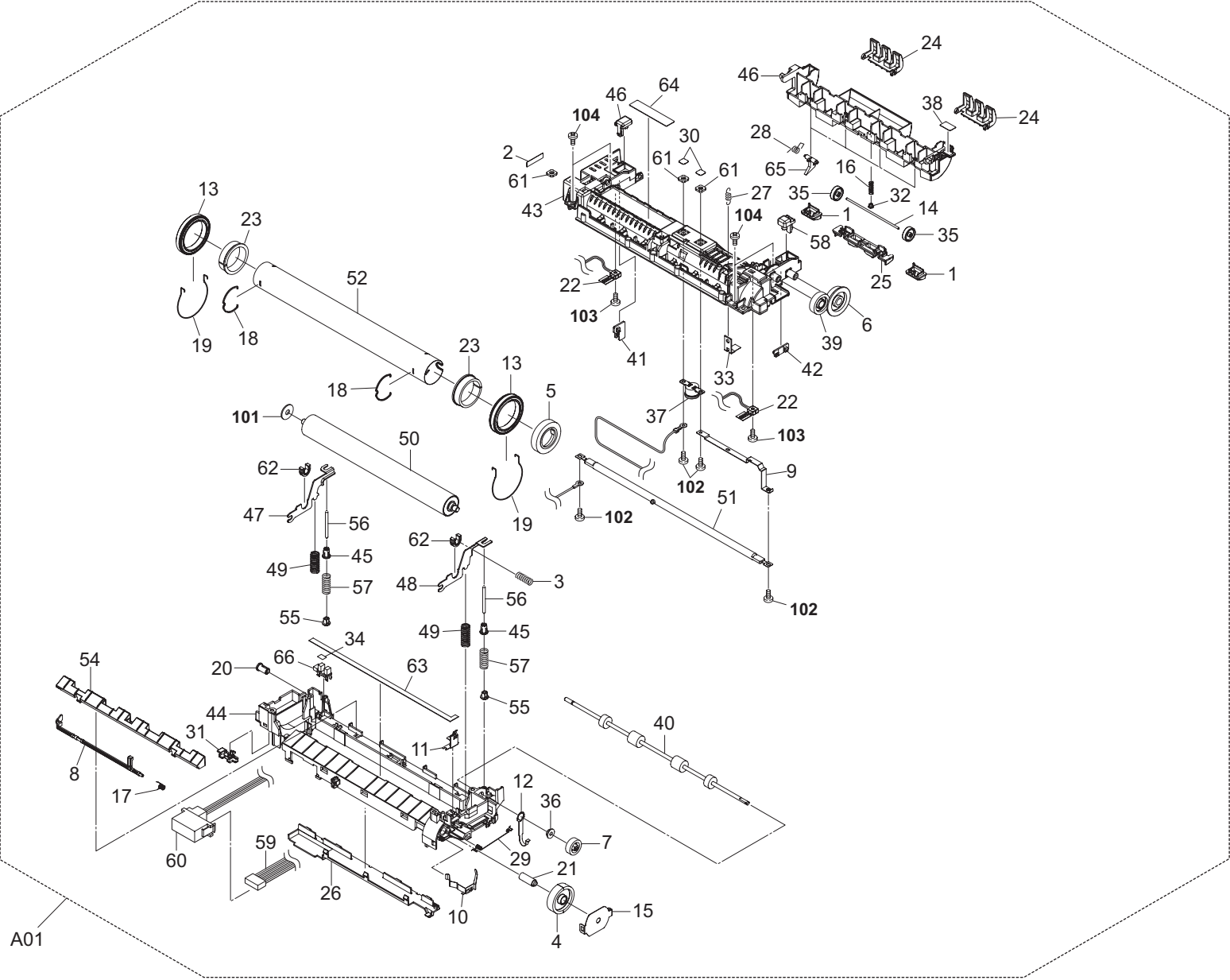
FIG. 11 Fuser Section 1 (FS-2020D)
