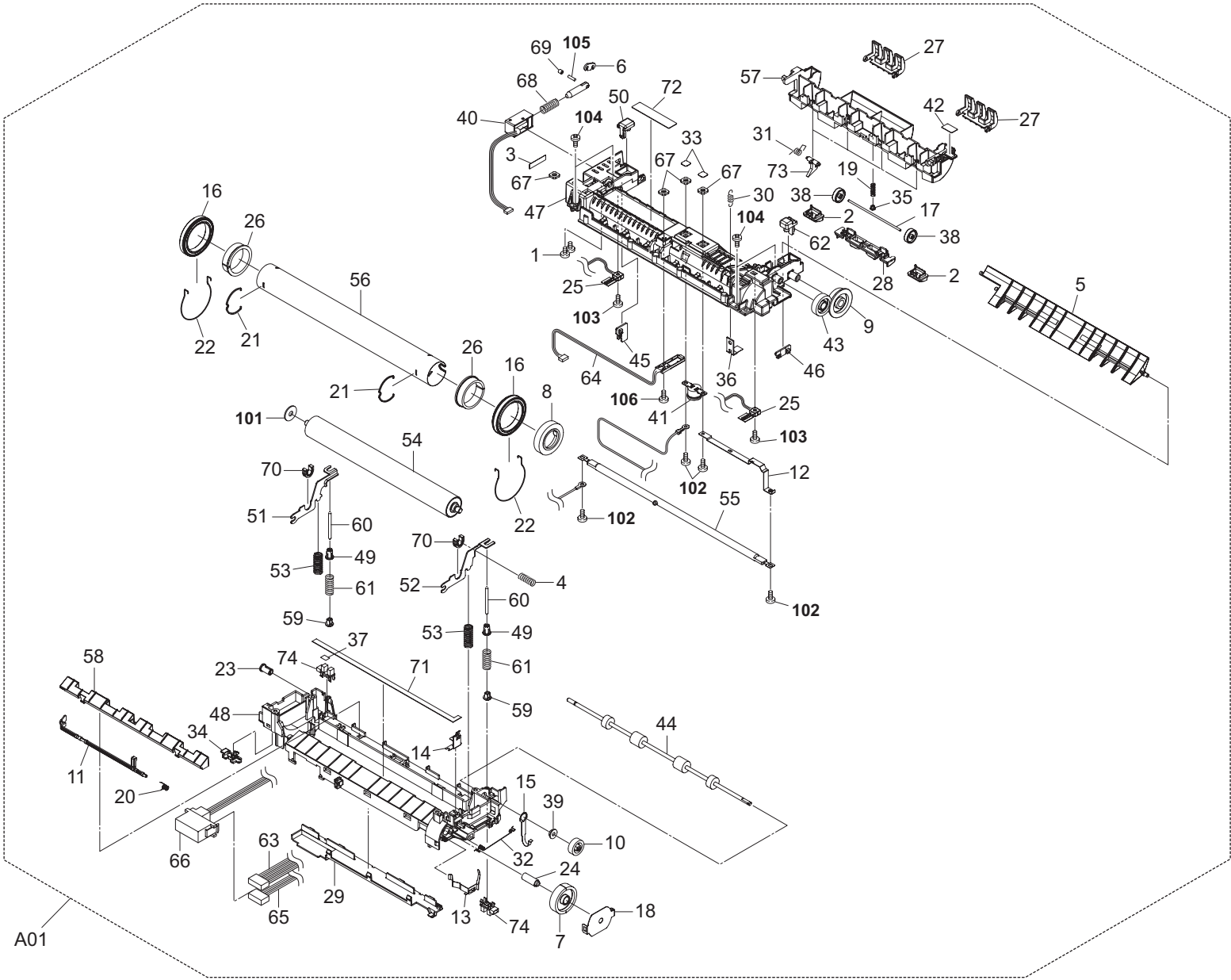
FIG. 11 Fuser Section 1 (FS-4020DN/3920DN)
