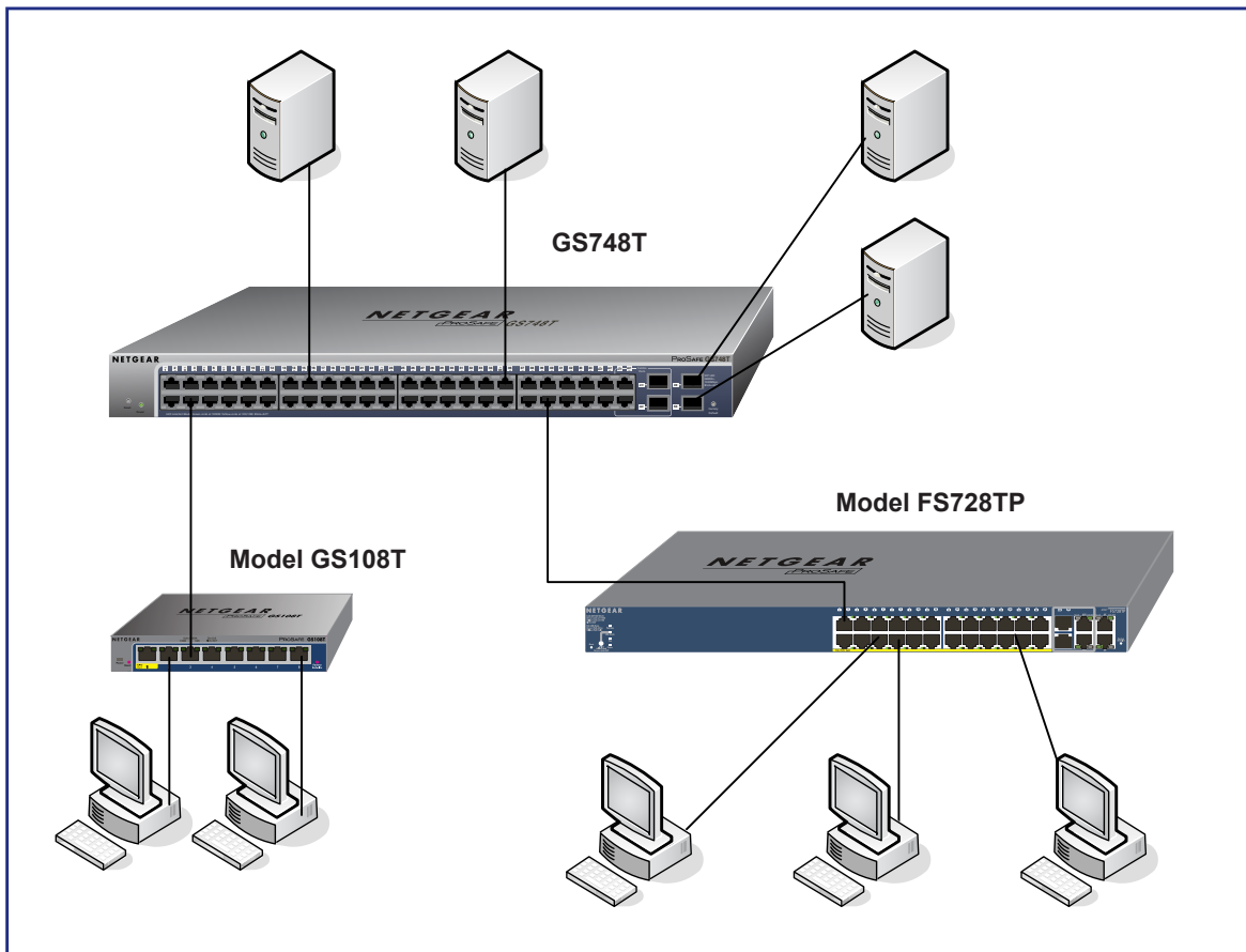
Figure 8. Backbone Switching
