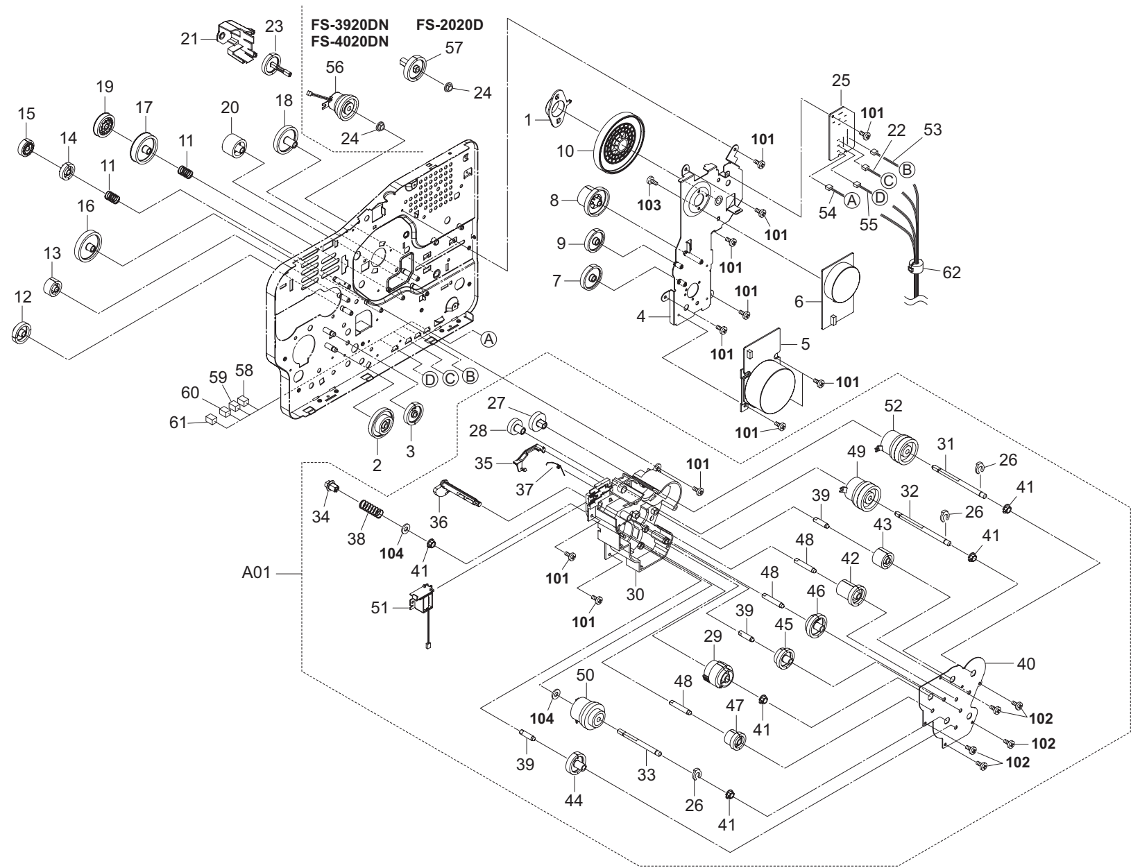
FIG. 13 Drive Section
