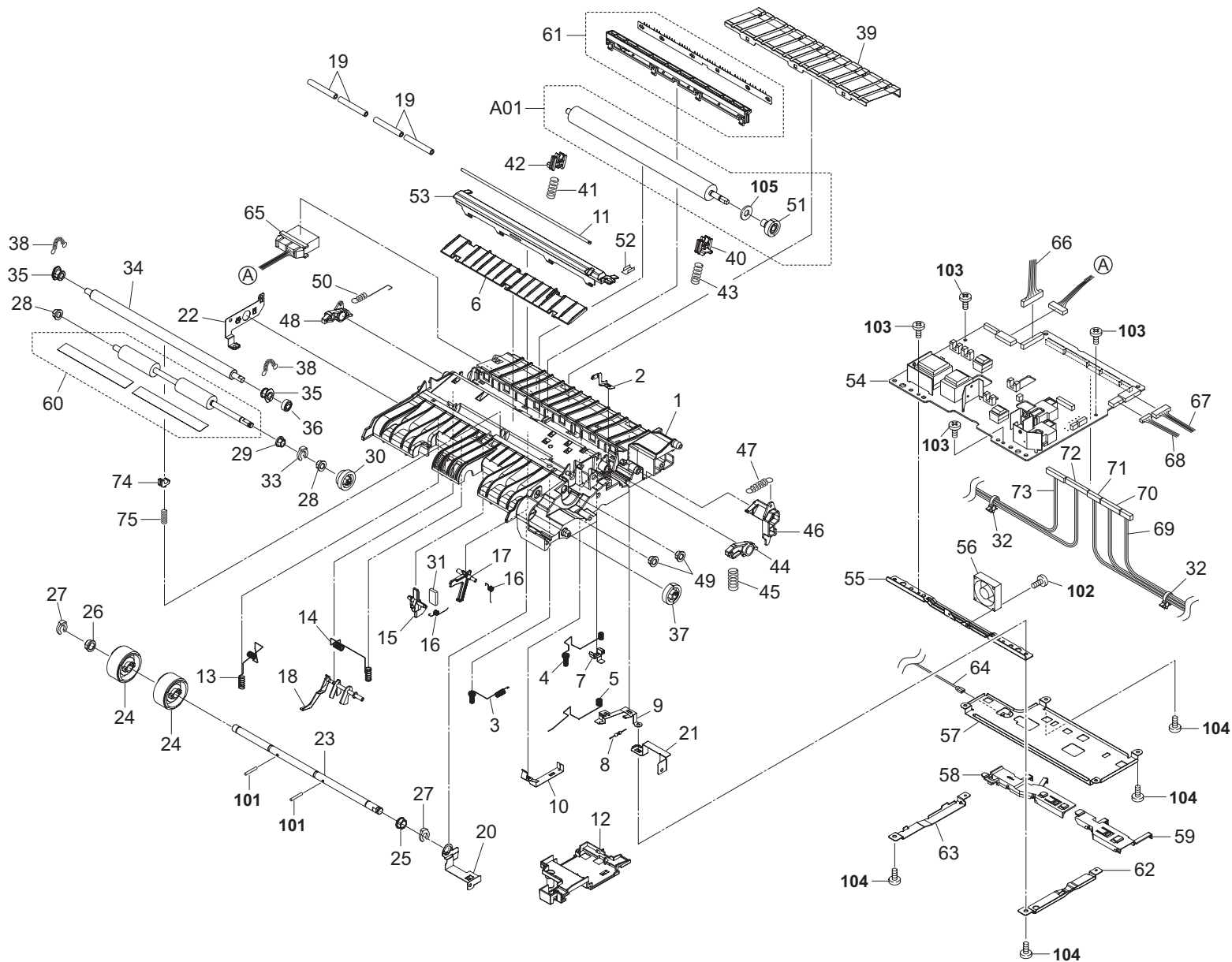
FIG. 6 Paper Feed Section 2
