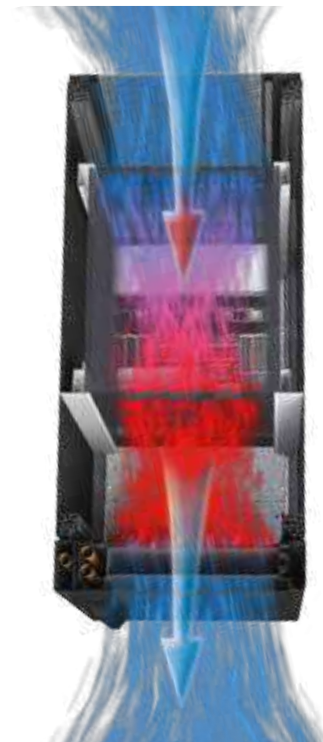
Server rack air flow with Knürr DCL (cross-section)
