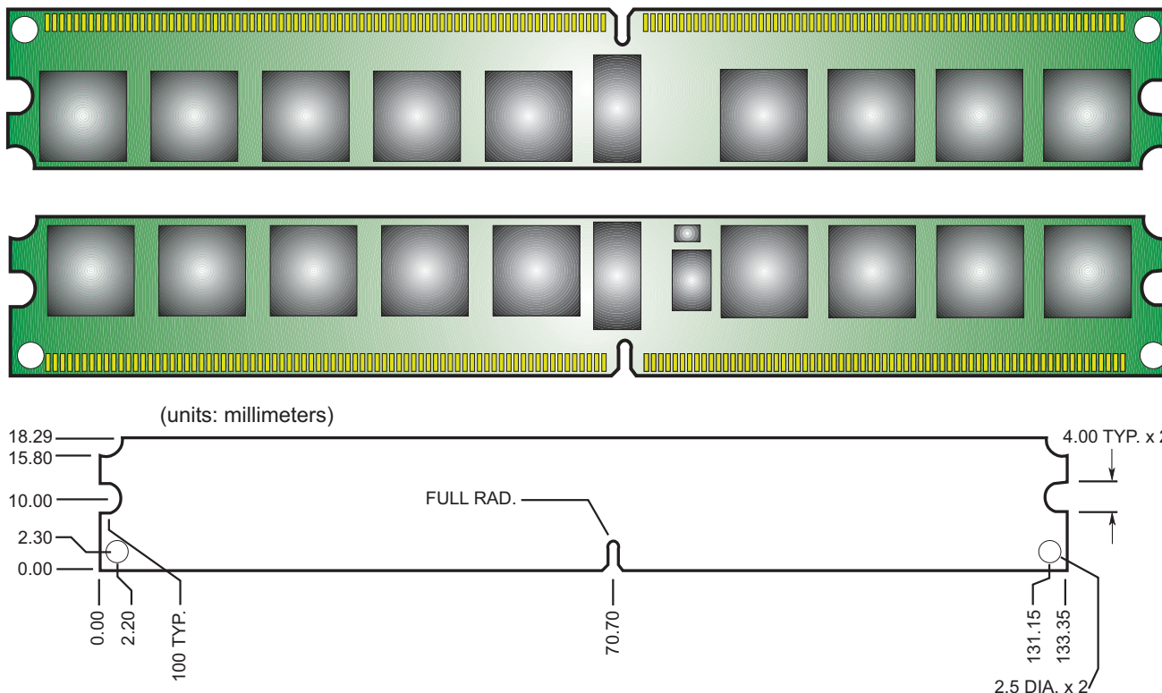
Figure 1: KVR667D2D8P5L/1G 240-Pin DIMM
