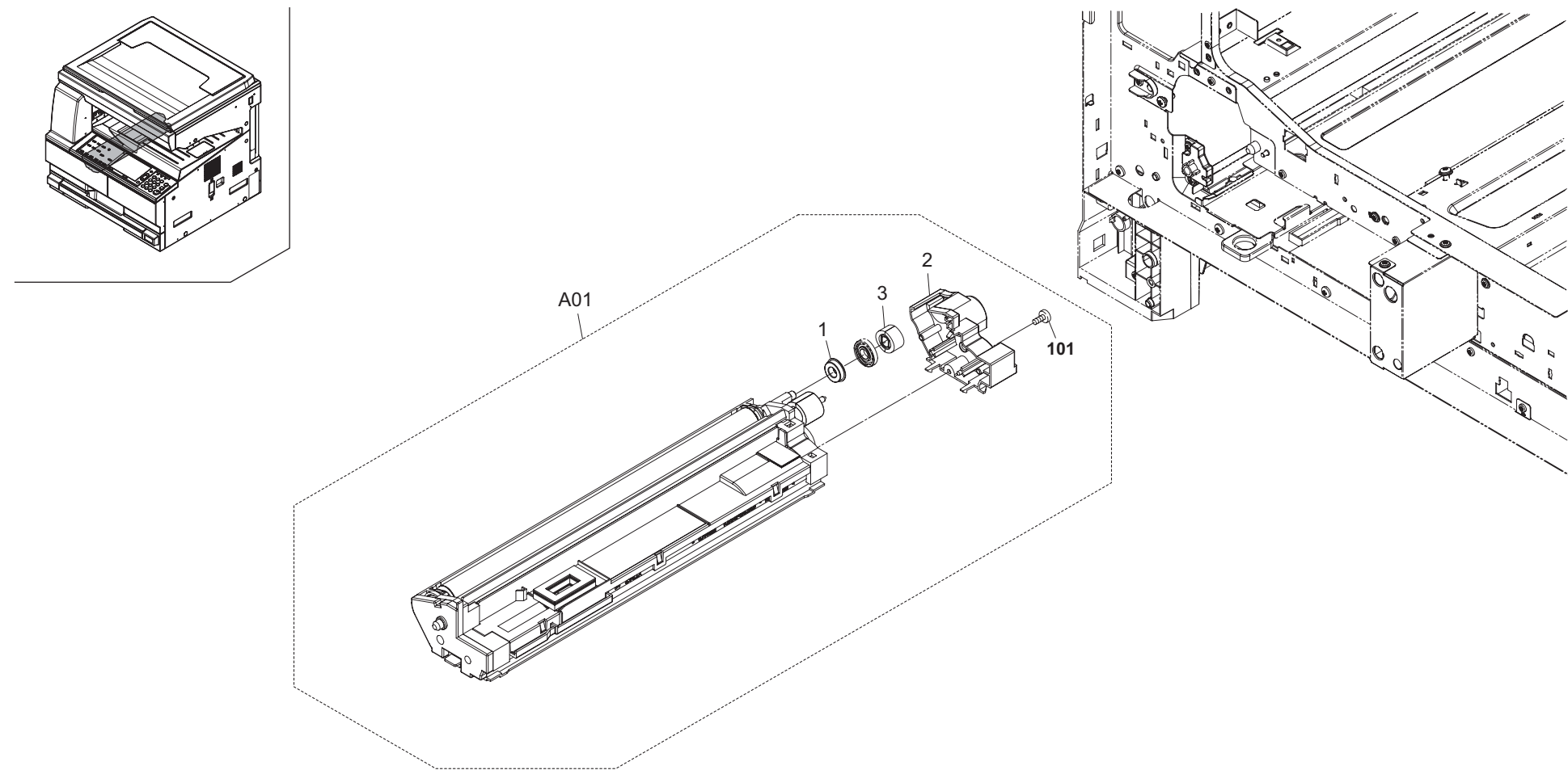
FIG. 11 Developing Section
