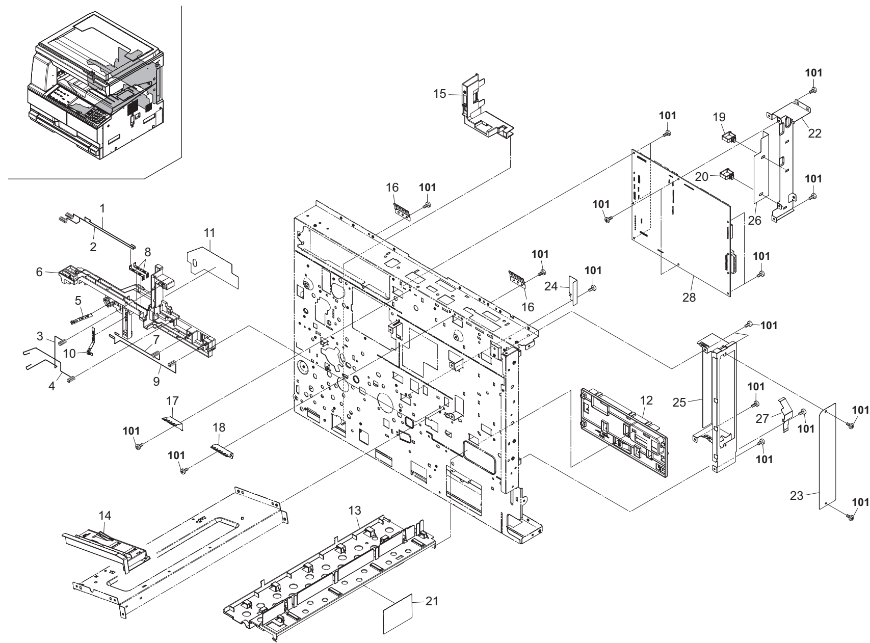
FIG. 18 Electrical Components 3
