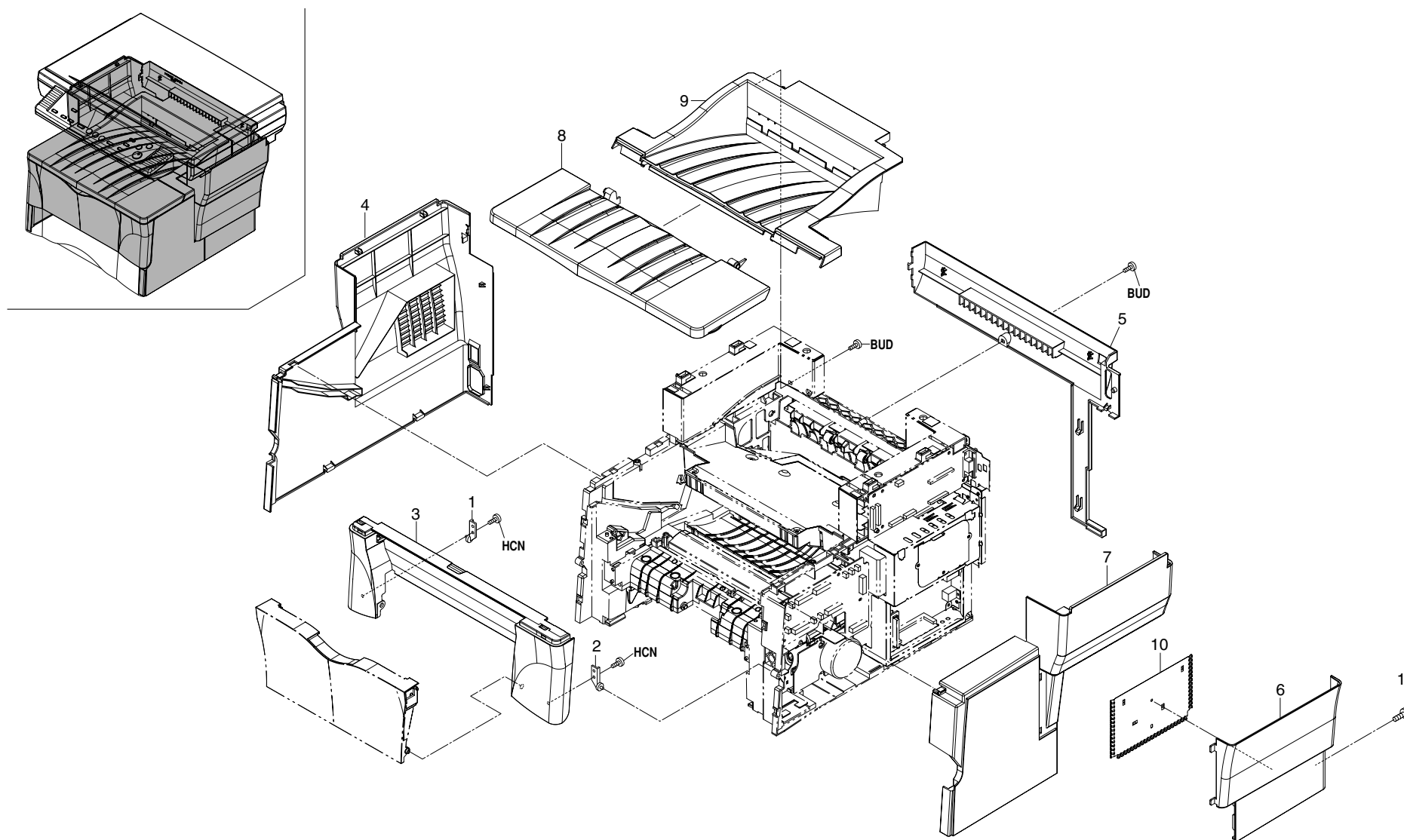
FIG. 1 EXTERIOR COVERS
