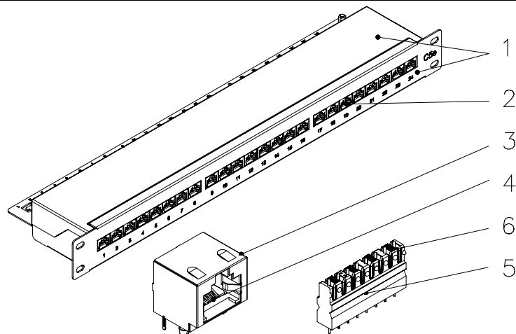
RJ45 RIGHT ANGLE JACK IDC Krone 45°-110 Dual
